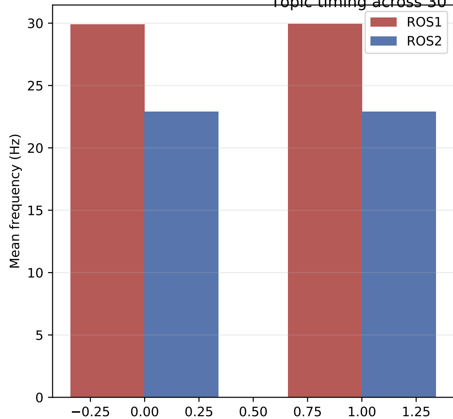
Topic timing across 30 matched runs per system
