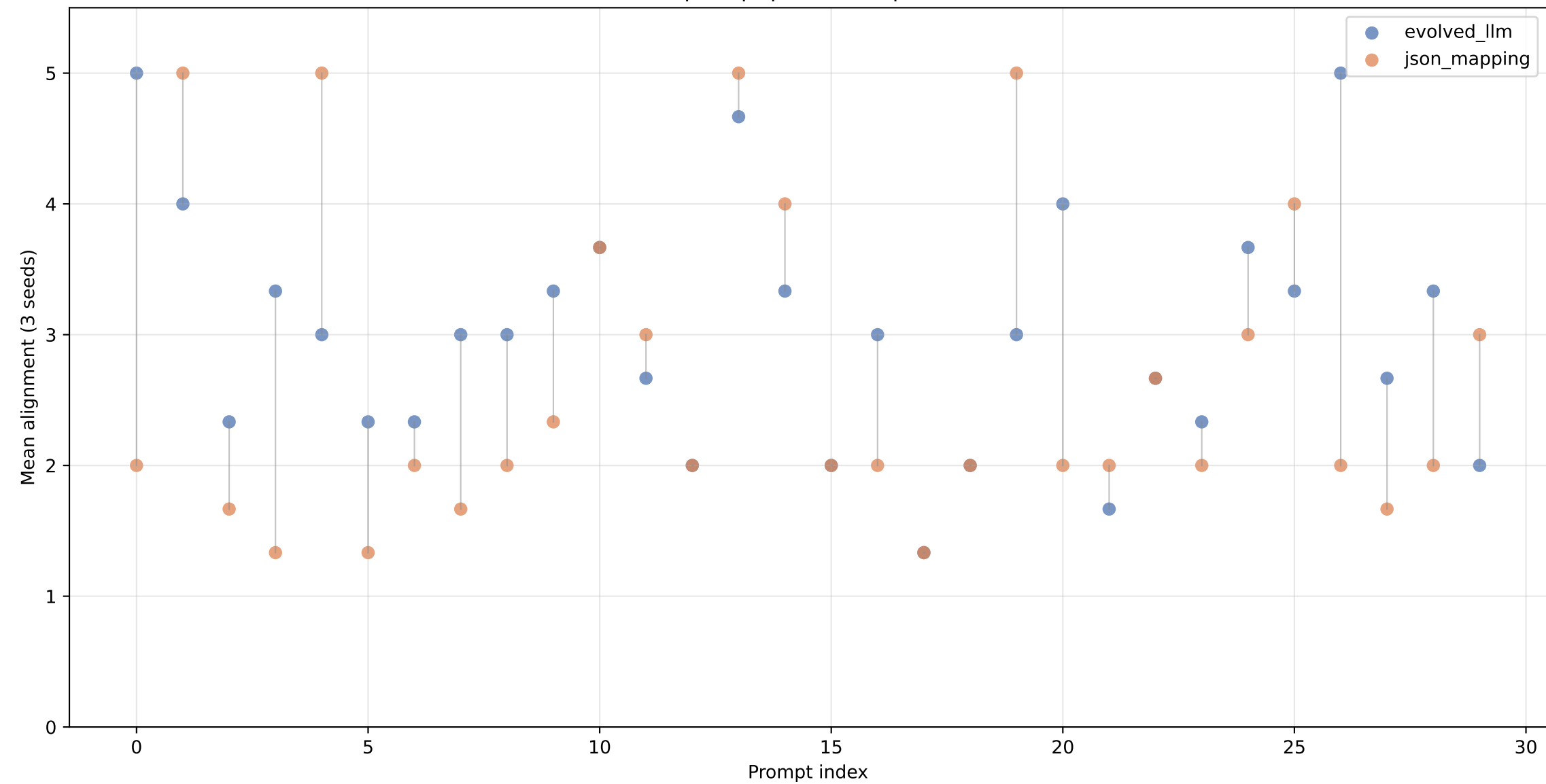
Per-prompt paired comparison
