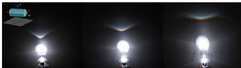
Fig. 4. Tangential arcs transitioning to the circumscribed halo for increasing light source inclinations ( 0^\circ – 30^\circ ), both produced by the mounted and turned-on module in Fig. 1(b). The lower tangential arc is covered by the machine in these pictures.
