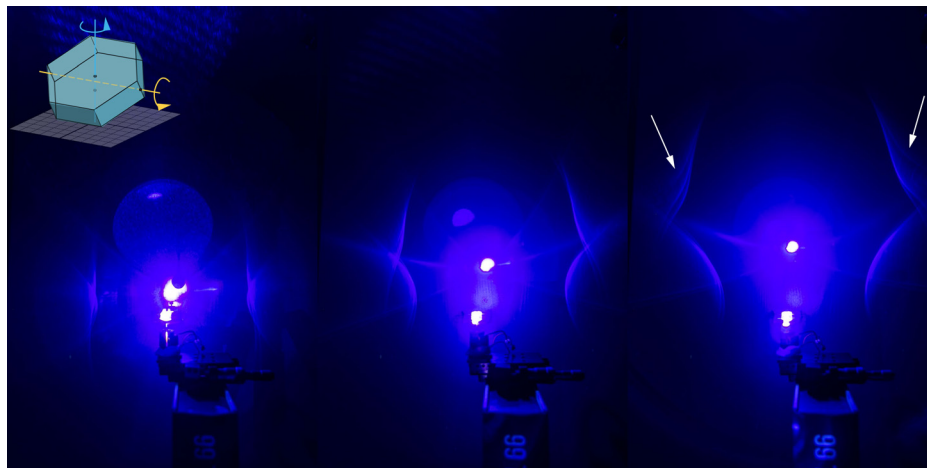
Fig. 3. Artificial Lowitz arcs (Ref. 13) generated by the mounted and spinning module in Fig. 1(a) with increasing light source inclinations ( 0^\circ – 30^\circ ). A low-power, focusable, blue laser diode ( \lambda = 405 nm, P < 1 mW) was used for illumination. The arrows indicate a faint feature/arcs appearing distinctly only at large elevations (Ref. 13).
