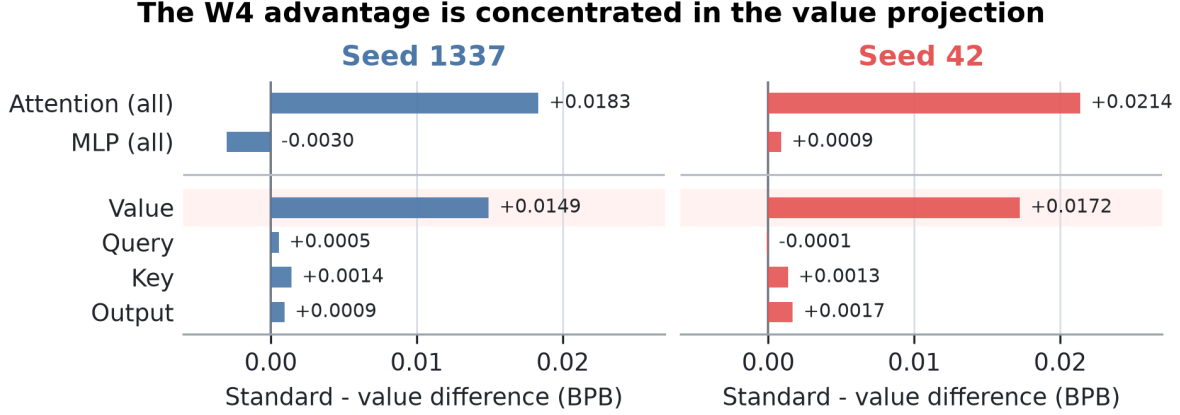
Figure 4: Standard-minus-value-difference damage by parameter group; positive values favor value differencing. Rows above the divider are whole modules; rows below it isolate projections within attention. Each bar is a separate intervention, so the effects need not add linearly.
