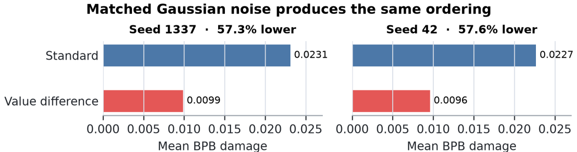
Figure 5: Mean BPB damage under RMSE-matched Gaussian perturbations of attention weights. Value differencing reduces damage by 57.3% and 57.6% across the two training seeds. The released control table reports all six paired noise realizations.
