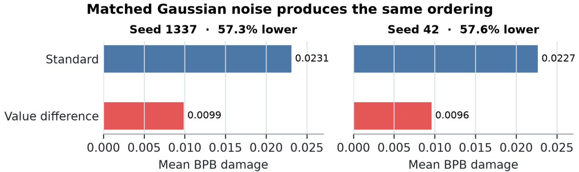
Figure 5: Mean BPB damage under RMSE-matched Gaussian perturbations of attention weights. Value differencing reduces damage by 57.3% and 57.6% across the two training seeds. The released control table reports all six paired noise realizations.
