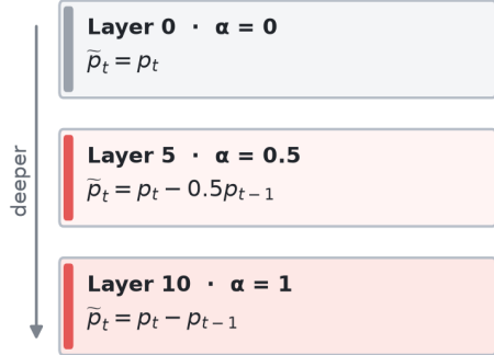
Figure 1: Value differencing changes only the payload supplied to attention. The same learned value projection processes the current and previous positions. The fixed coefficient \alpha_\ell grows with depth, moving from raw values to full previous-token differences; queries and keys are unchanged.
