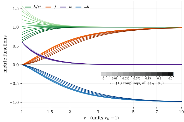
Figure 1: The four amplitudes of the equal-spin ansatz at all 13 couplings, \alpha = 0 (lightest) to \alpha = 1/2 (darkest), at spin q = 0.6 and r_H = 1 ; each curve is one nonlinear solve. Conventions follow fig. 1 of arXiv:1010.0860 : h is drawn as h/r^2 , which tends to unity at infinity, and b as -b , since b and f otherwise overlap.
