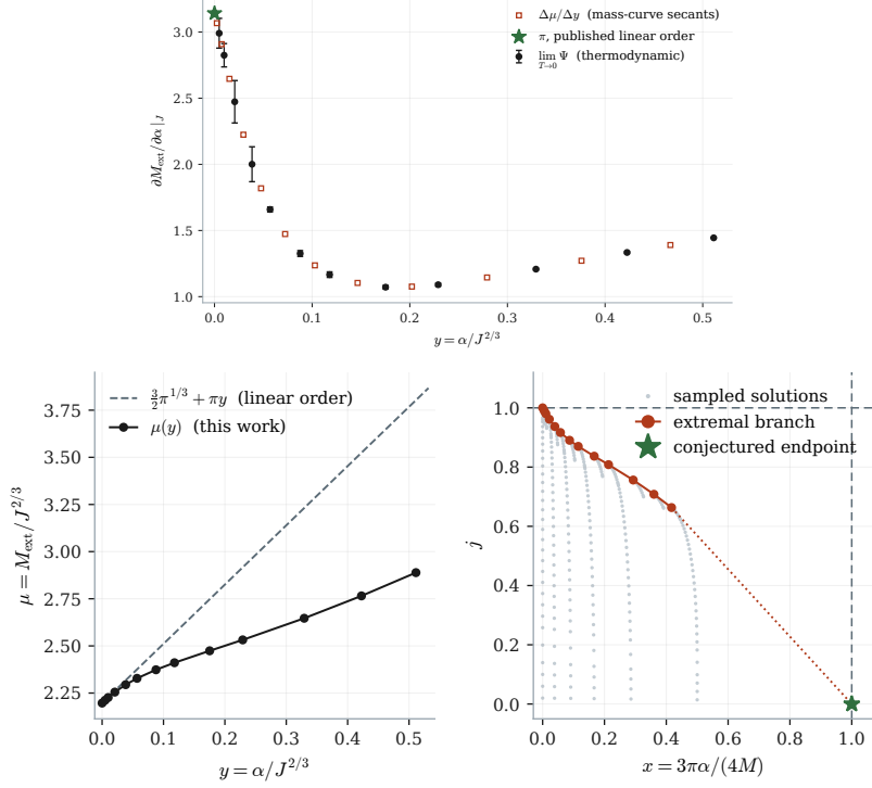
Figure 3: Top: the measured slope against y = \alpha/J^{2/3} , with the published linear-order value \pi as a star and secants of the mass curve as open squares. Bottom left: the extremal mass the slope integrates to, against the first-order line. Bottom right: the same branch in the (x, j) domain-of-existence plane of arXiv:2303.12471 . Circles are T = 0 intercepts of fits, not constructed solutions.
