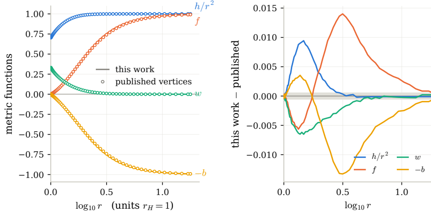
Figure 2: Left: the four metric functions at \alpha_{\text{ref.}} = 3 , q = 0.33 , ours as lines and as markers the 74 vertices read from fig. 1 of Brihaye, Kleihaus, Kunz and Radu, arXiv:1010.0860 . Right: the difference, with the band of one device unit of that figure ( 5.17 \times 10^{-4} ) shaded. Conventions as in fig. 1, which is what makes the two directly comparable.
