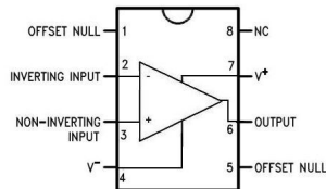
LM741 Pinout Diagram
