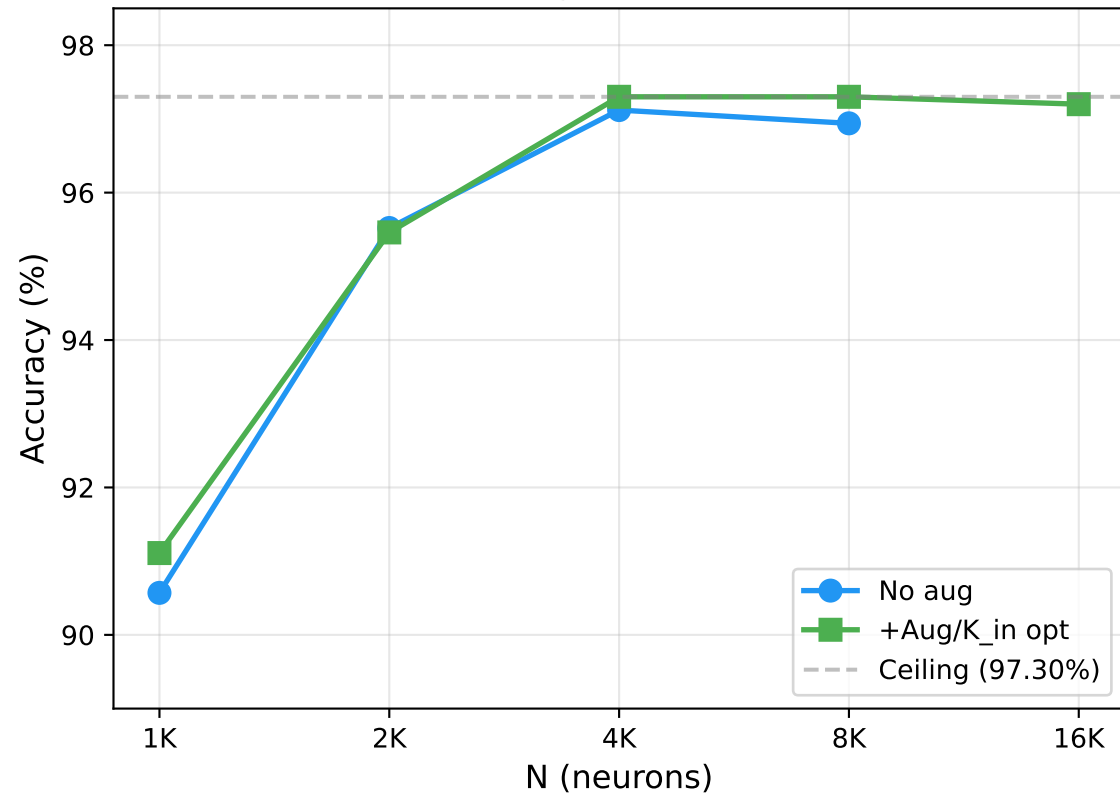
Imagenette T2
