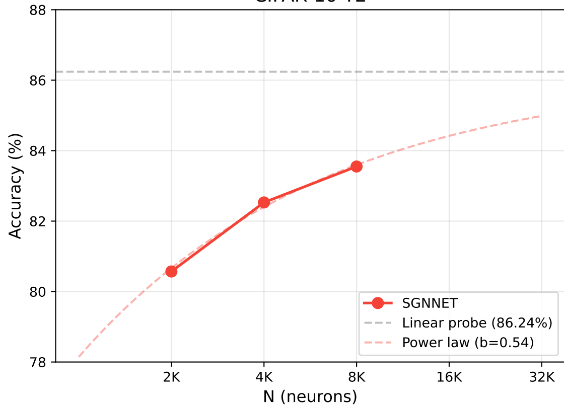
CIFAR-10 T2
