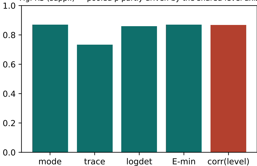
Fig. R3 (suppl.) — pooled \rho partly driven by the shared level axis
