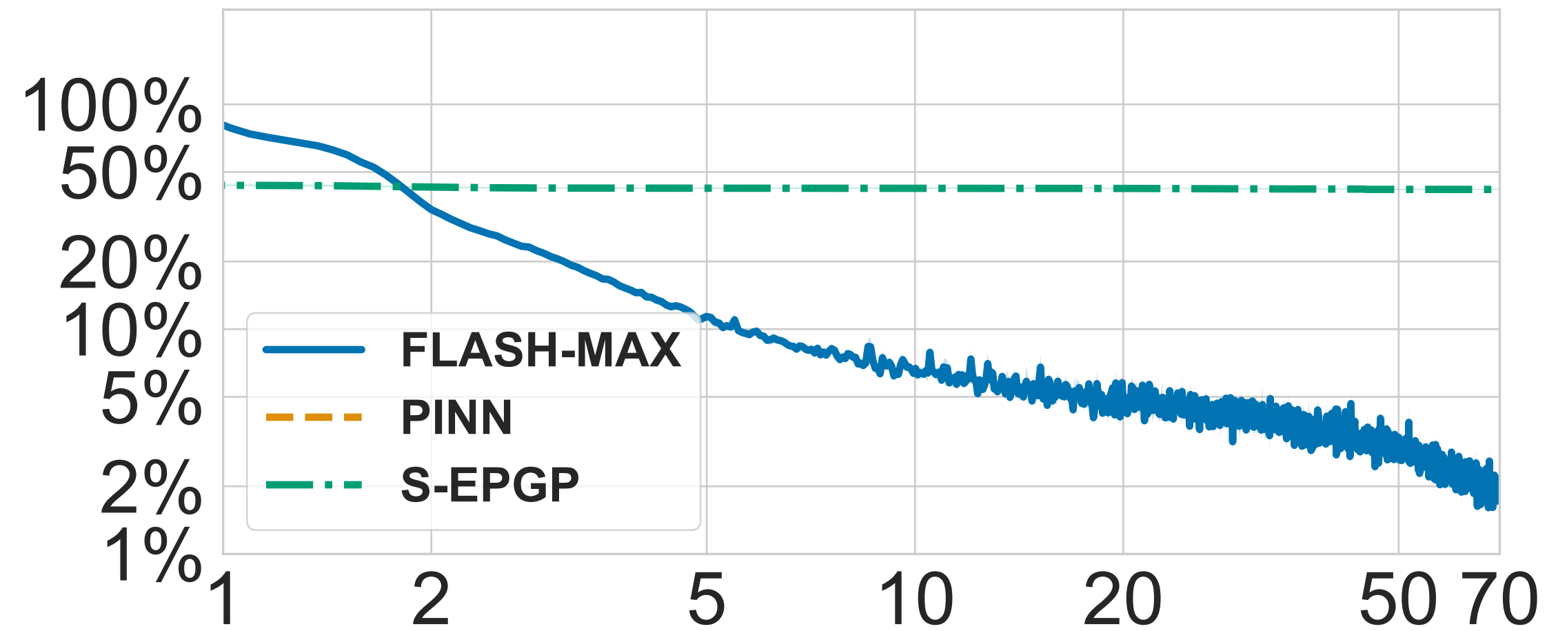
Random solution
