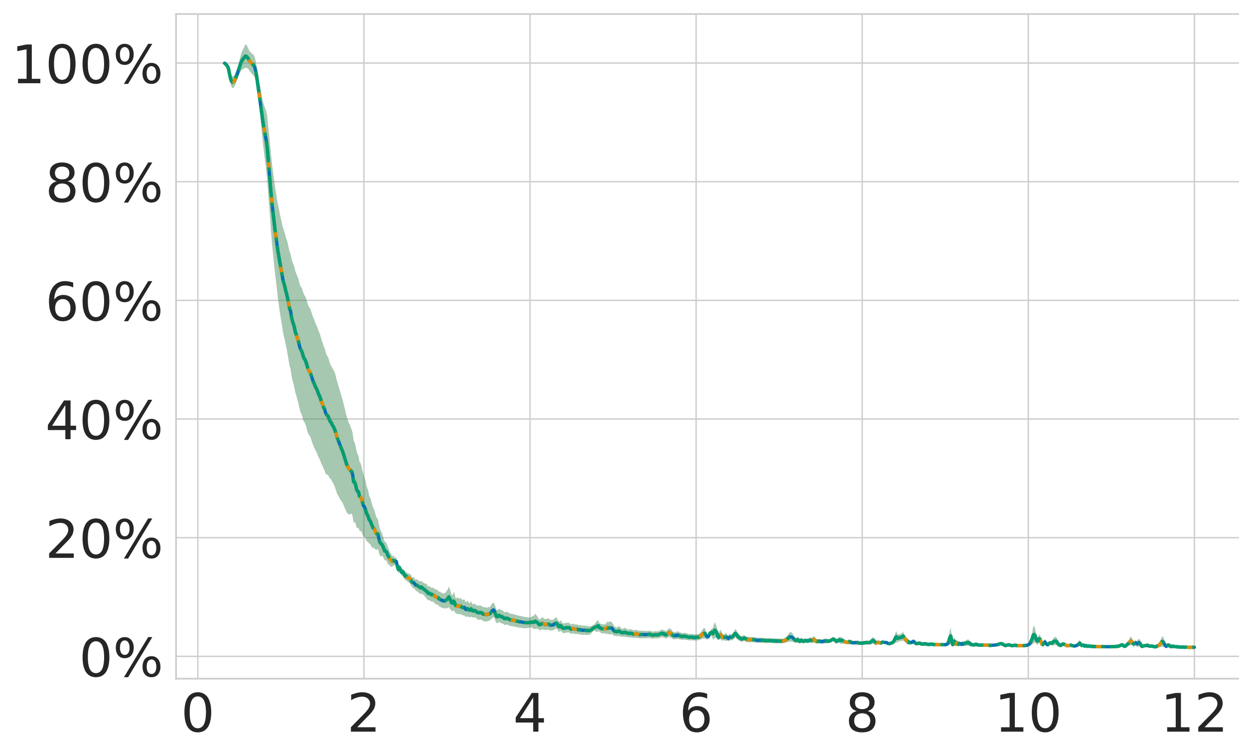
Radial waves
