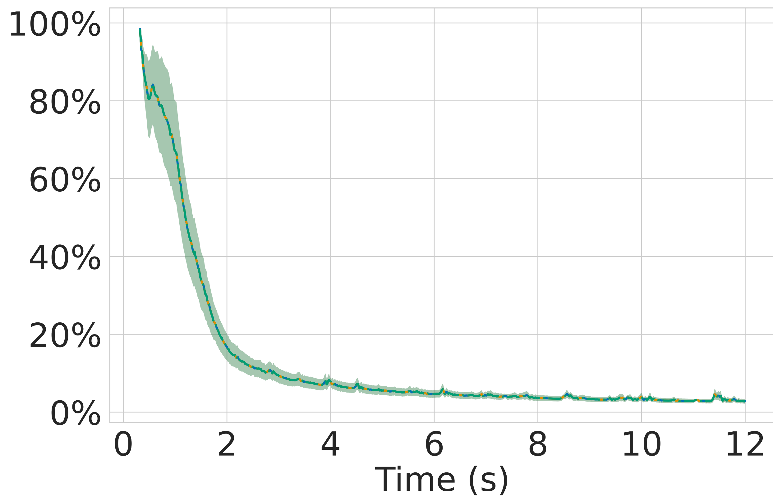
Random solution
