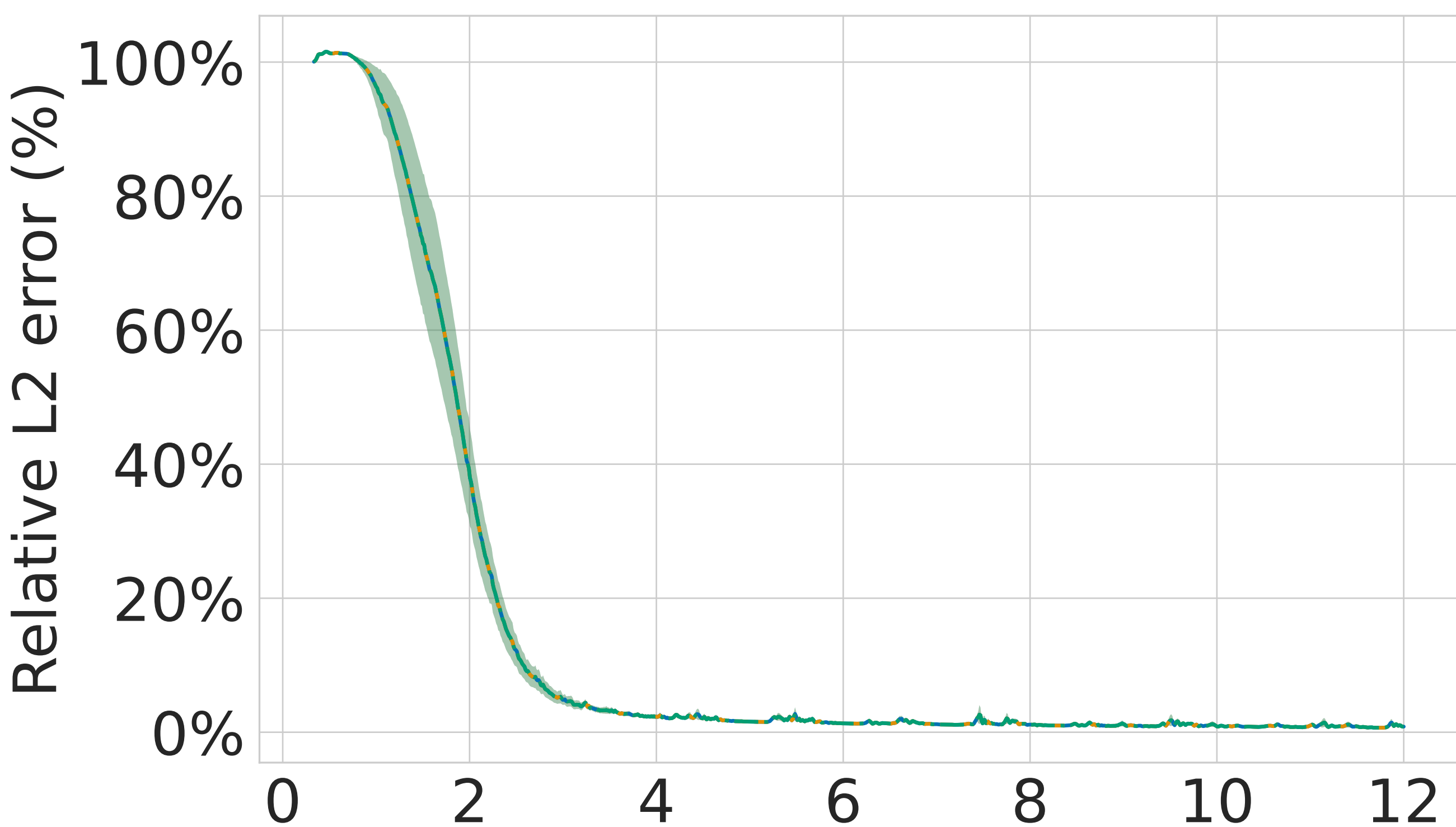
Plane waves
