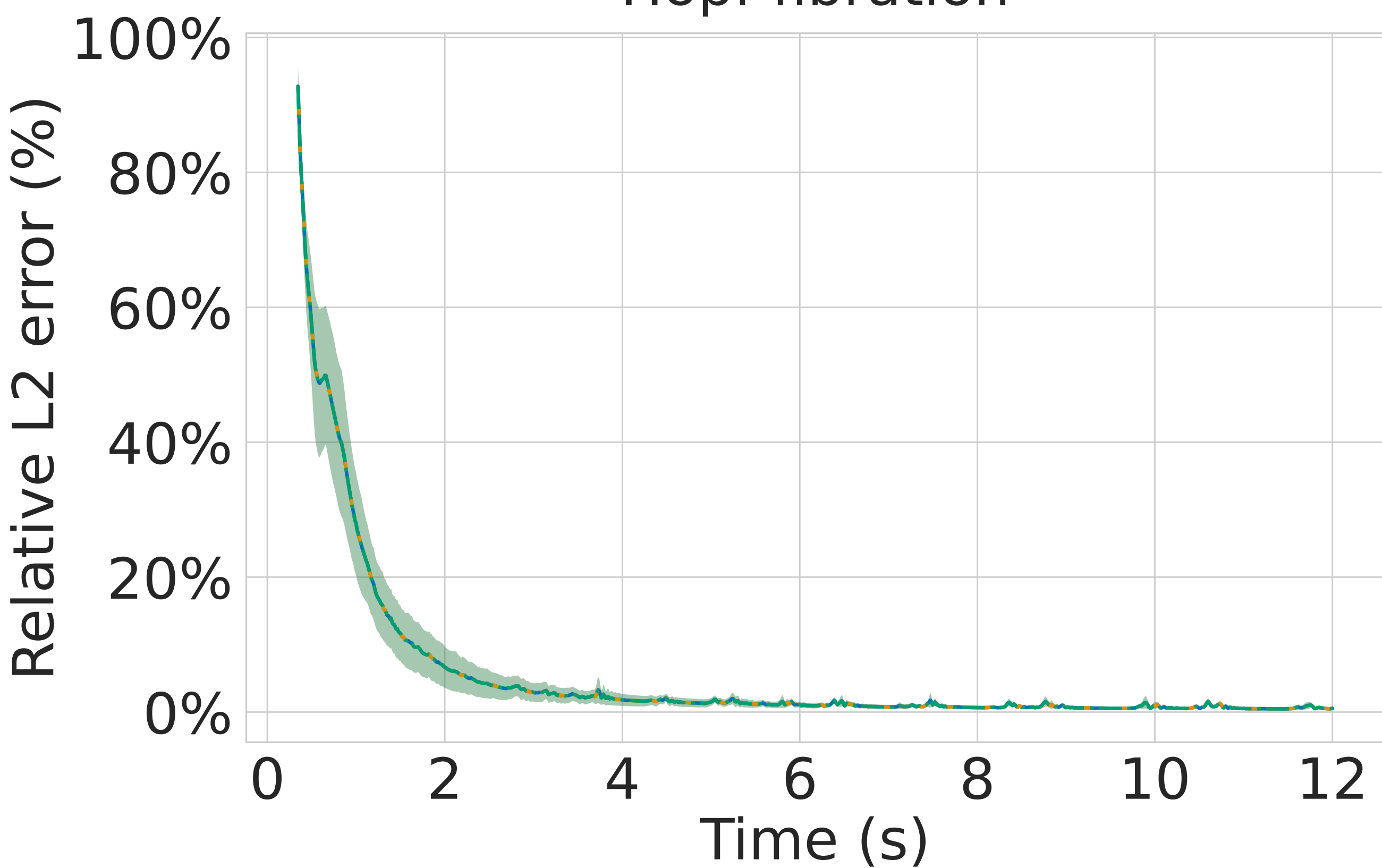
Hopf fibration
