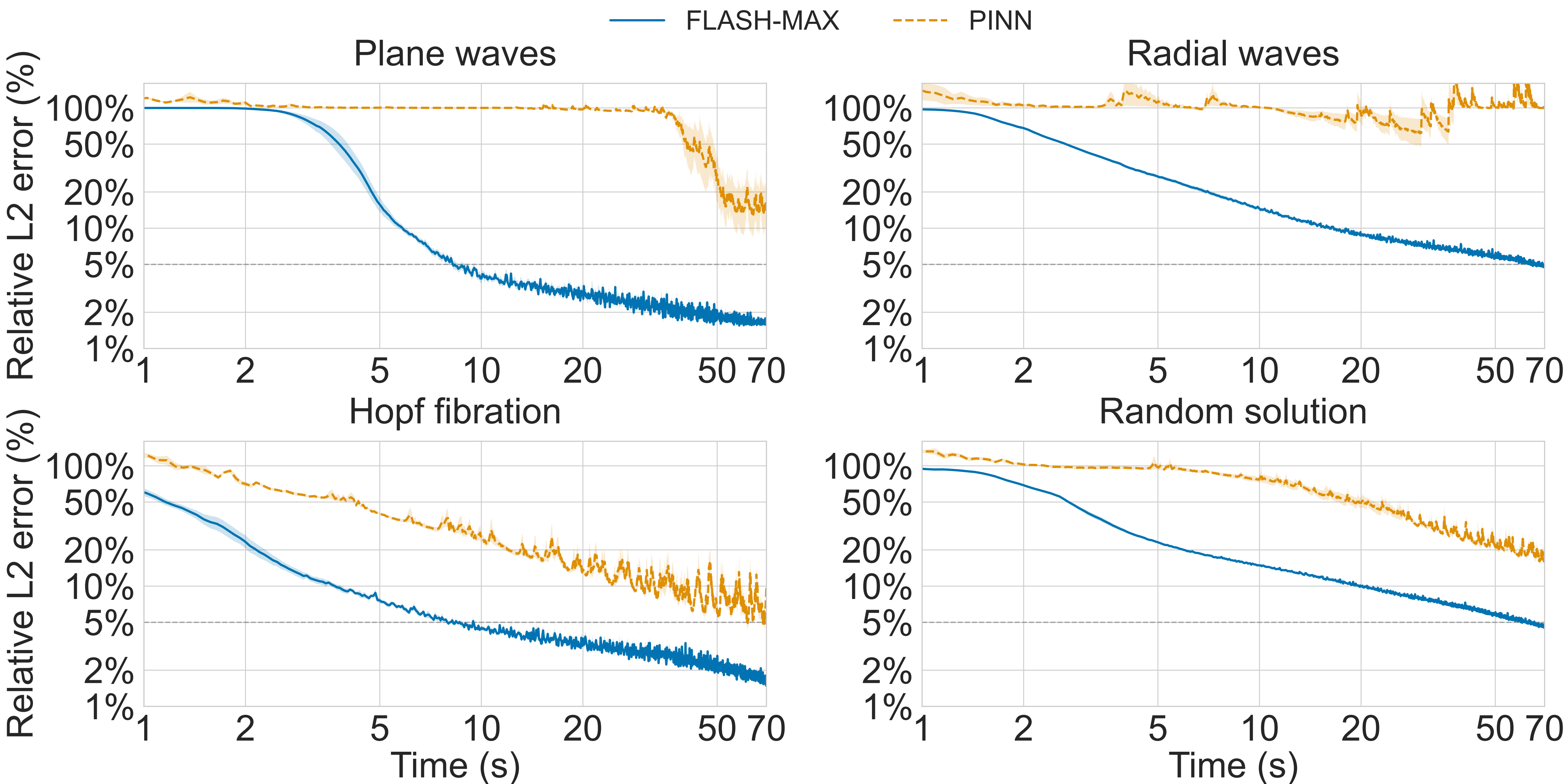
Relative L2 validation error over time (w/ BC on NVIDIA L40S, average of 5 seeds), log-log scale
