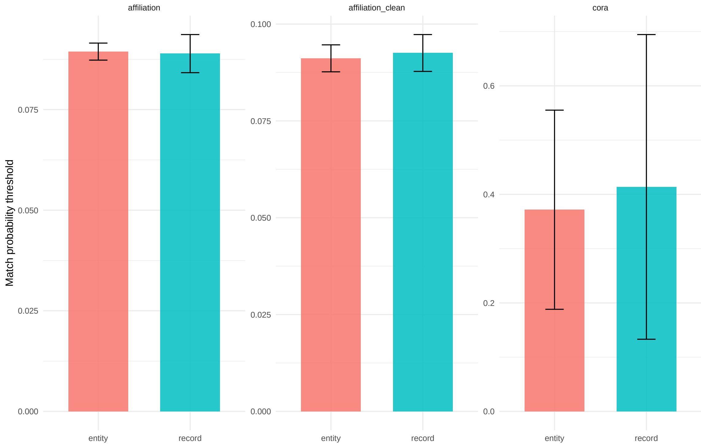
Decision threshold by dataset and split strategy
