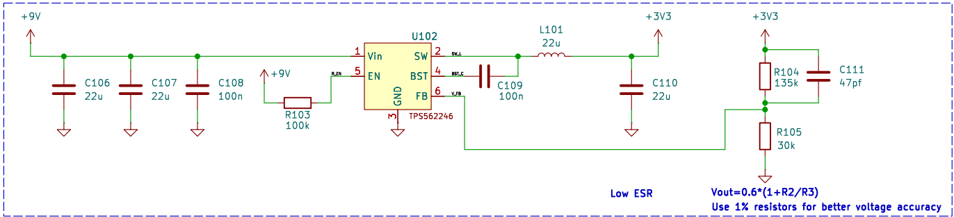
Digital Supply
