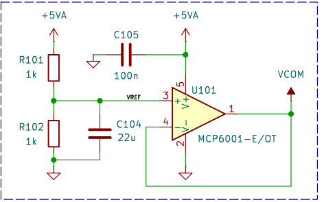
Bias Generator
