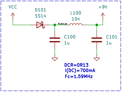
Input filter + reverse polarity protection
