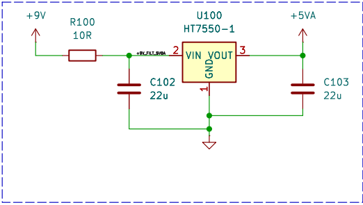
Analogue supplies
