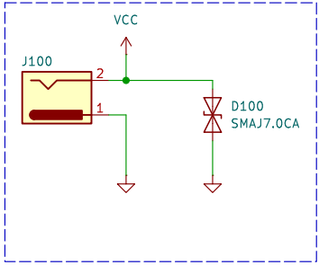
Power connector
