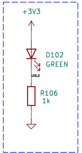
Power LED
