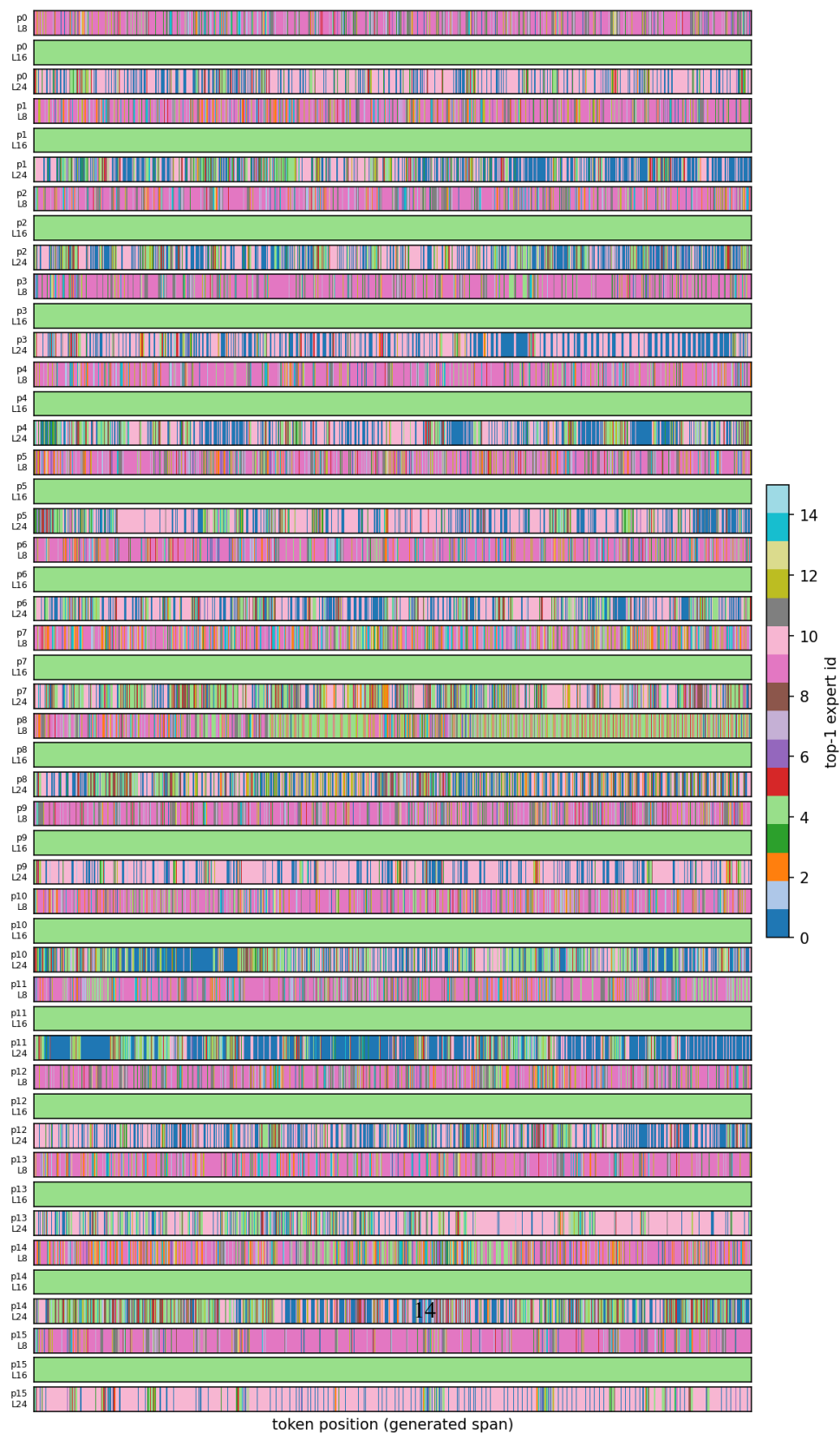
Figure 6: Phi-tiny-MoE-instruct, option-critic-controller-baseline, expert routing trace at layers 8/16/24
