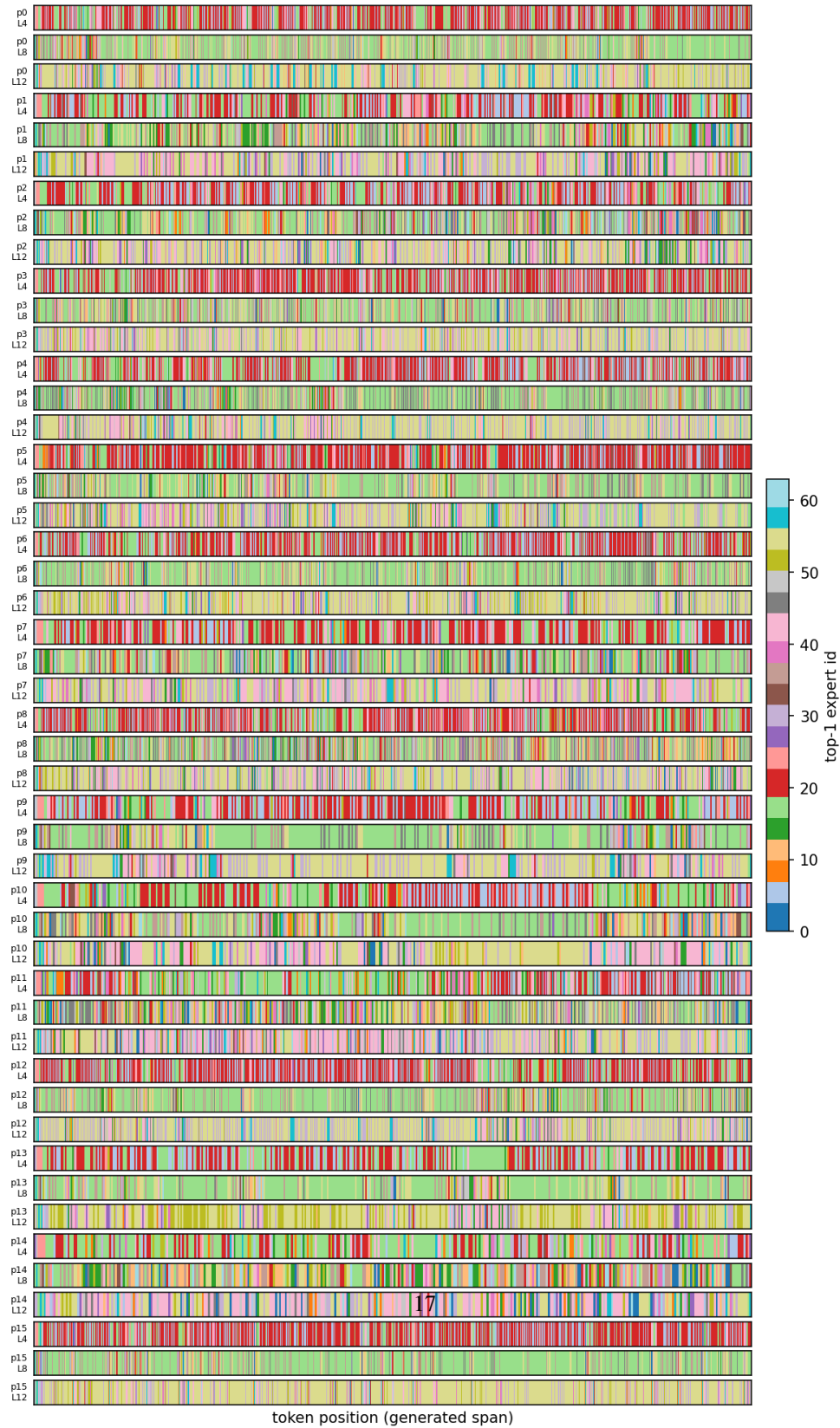
Figure 9: OLMoE-1B-7B_causal LM alone (SFT) - expert routing trace at layers 4/8/12
