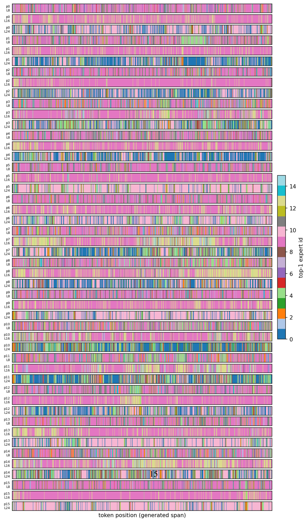
Figure 7: Phi-tiny-MoE-instruct, MELINOE baseline, expert routing trace at layers 8/16/24
