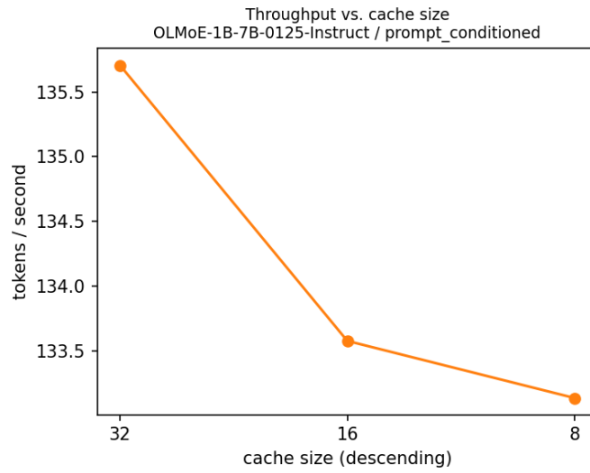
Figure 14: OLMoE-1B-7B, prompt-conditioned policy – estimated tokens/second (own, adapter-inflated measurement, not base-normalized) as a function of the conditioned capacity c \in \{8, 16, 32\} (descending on the x -axis), corresponding to Table 3.
