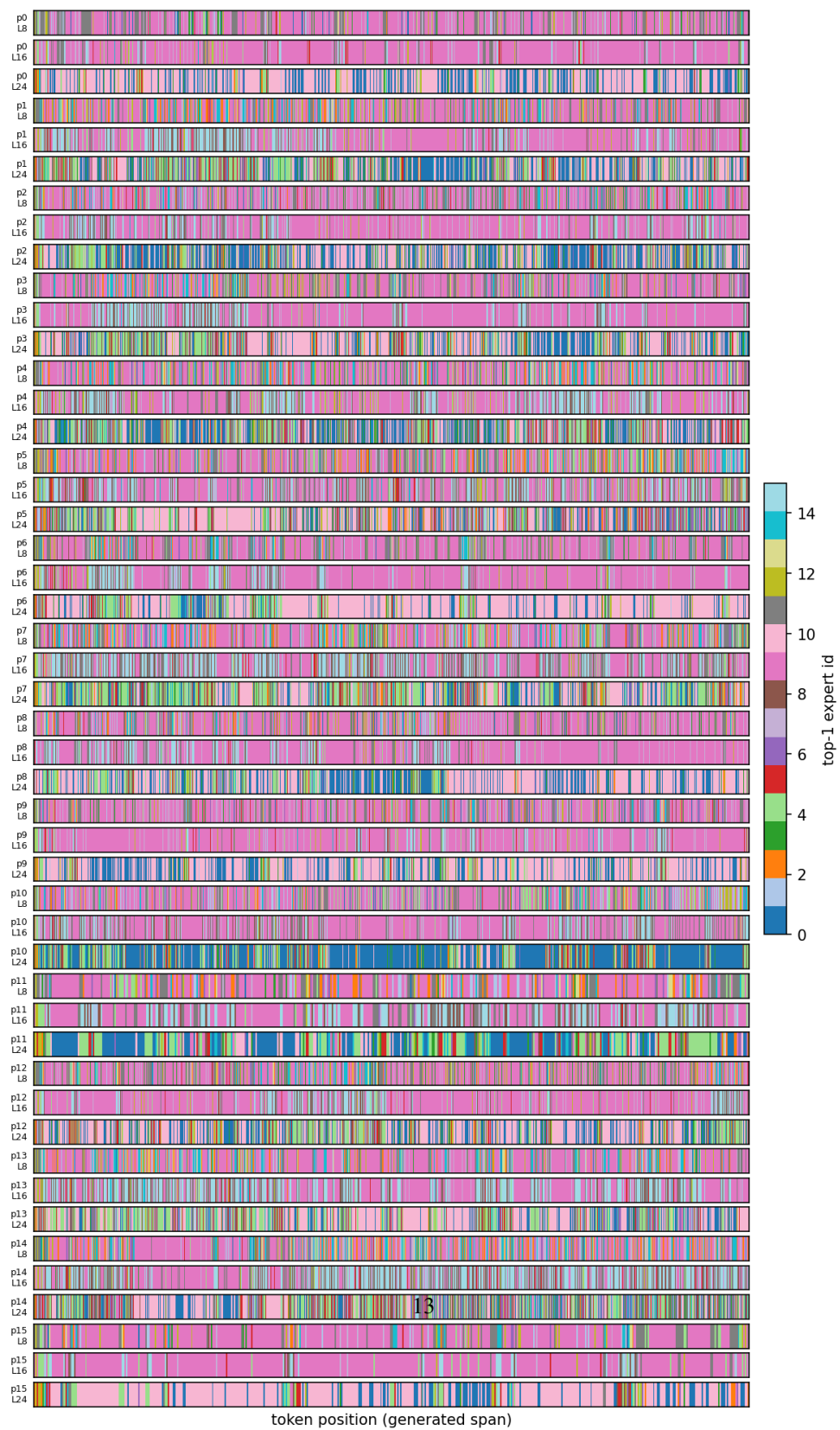
Figure 5: Phi-tiny-MoE-instruct, working-set reward + SET (combined objective) expert routing trace at
