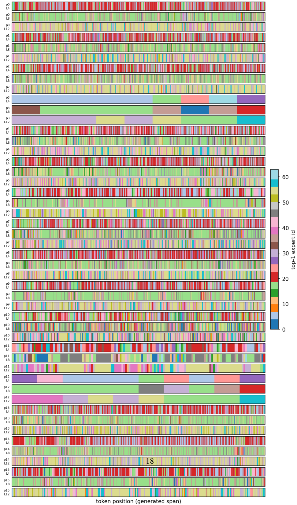
Figure 10: OLMoE-1B-7B, working set reward alone – expert routing trace at layers 4/8/12
