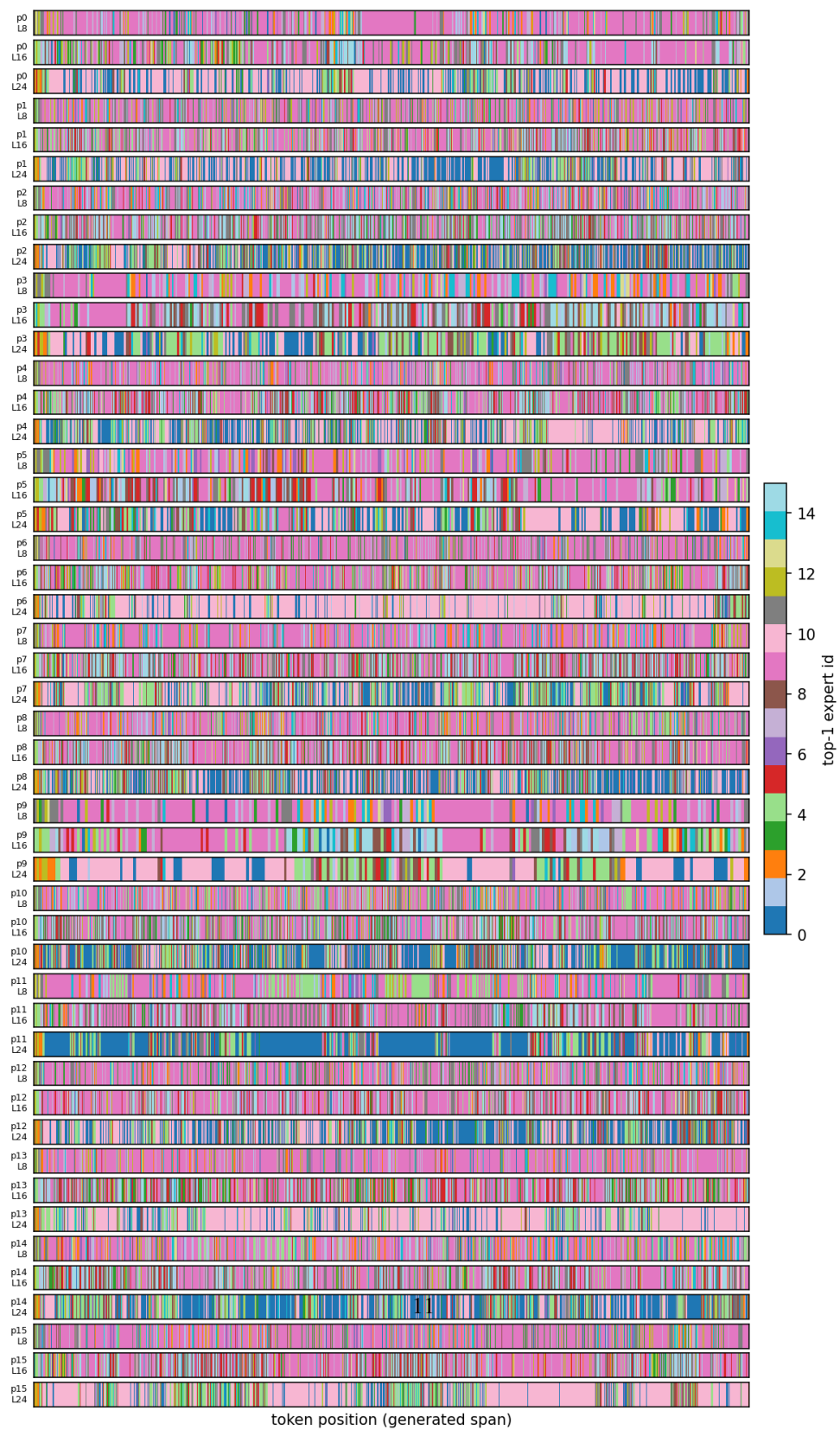
Figure 3: Phi-tiny-MoE-instruct-causal LM alone (SET) - expert routing trace at layers 8/16/24
