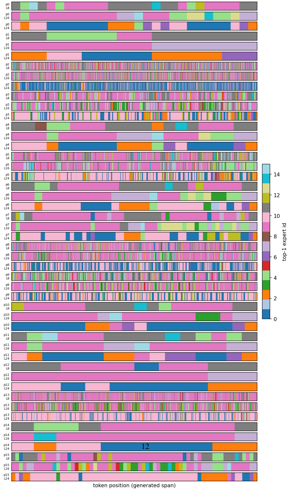
Figure 4: Phi-tiny MoE-instruct, working set reward alone – expert routing trace at layers 8/16/24
