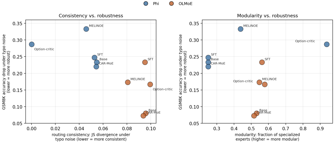
Figure 1: Left: routing consistency (JS divergence under typo noise) vs. GSM8K accuracy drop under the same perturbation. Right: modularity (fraction of specialized experts) vs. the same accuracy drop. Within each backbone, CAR-MoE and Base/SFT cluster together; Phi-tiny-MoE’s option-critic controller (labeled) is the outlier in both panels – maximally consistent and maximally "specialized," yet the least robust objective on this backbone.
