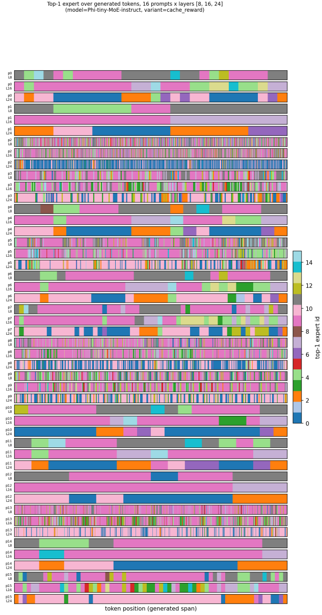
Figure 4: Phi-tiny-MoE-instruct, working-set reward alone – expert routing trace at layers 8/16/24.
