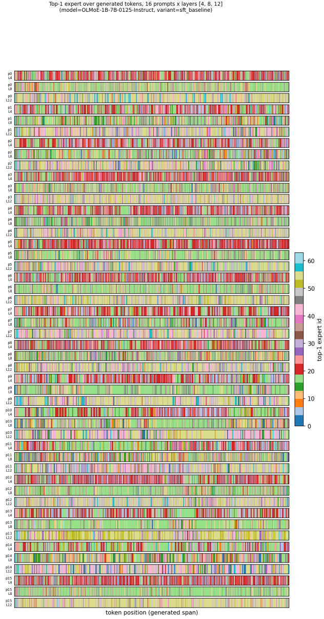
Figure 9: OLMoE-1B-7B, causal LM alone (SFT) – expert routing trace at layers 4/8/12.
