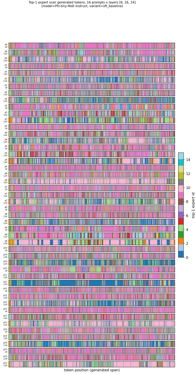
Figure 3: Phi-tiny-MoE-instruct, causal LM alone (SFT) – expert routing trace at layers 8/16/24.
