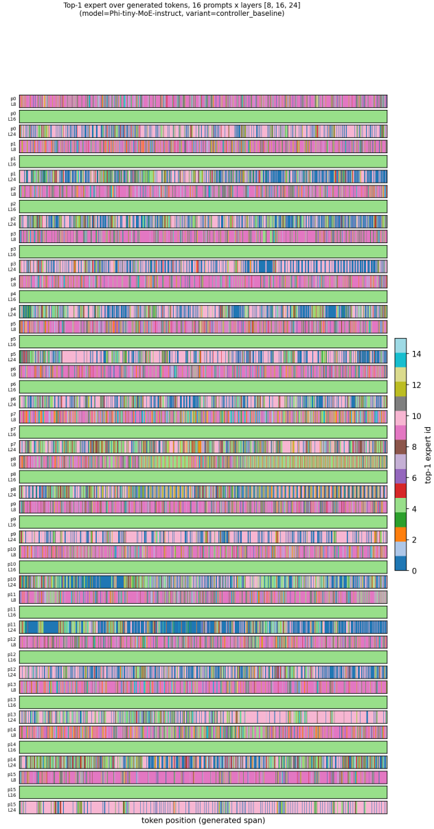
Figure 6: Phi-tiny-MoE-instruct, option-critic controller baseline – expert routing trace at layers 8/16/24.
