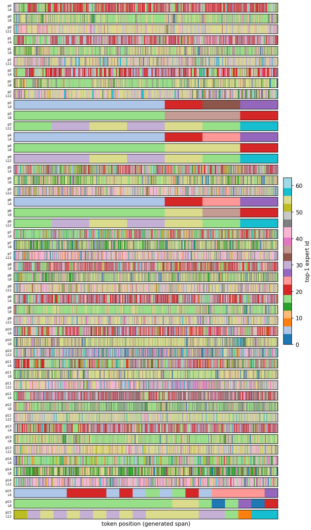
Figure 12: OLMoE-1B-7B, MELINOE baseline – expert routing trace at layers 4/8/12.
