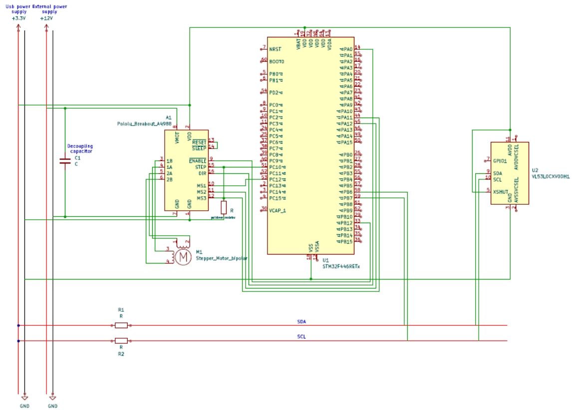
Figure 6: Kicad hardware electrical scheme
