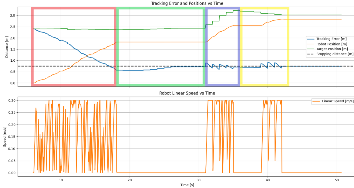
Figure 6: Tracking Error and Robot Linear Speed vs Time
