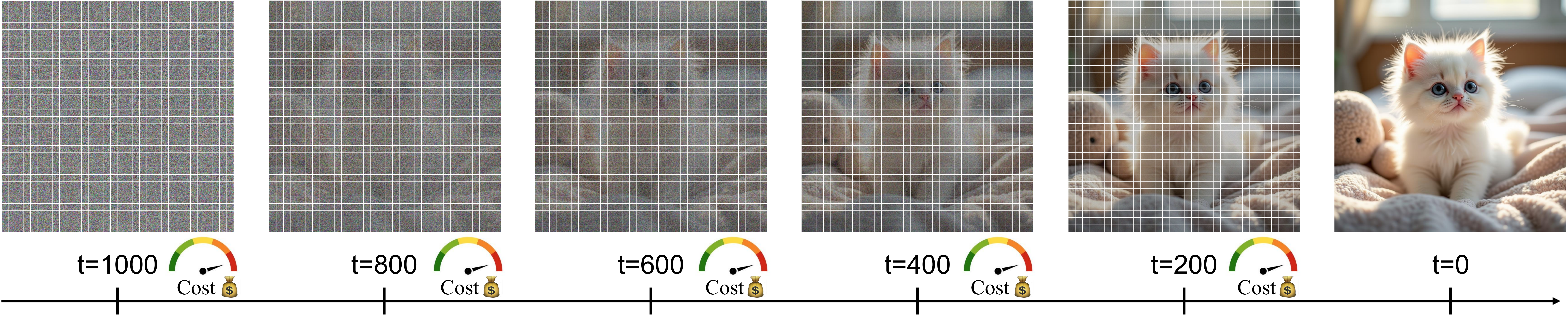
(a) Denoising process of standard diffusion transformers (DiTs)
