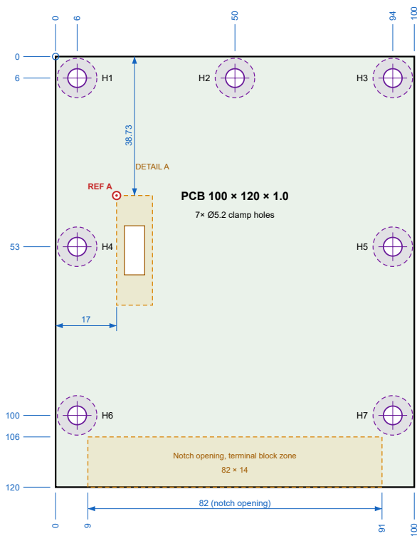
CCTV-8CH ENCLOSURE PCB OUTLINE — REV D (7 × Ø5.2 CLAMP HOLES, REF A)
