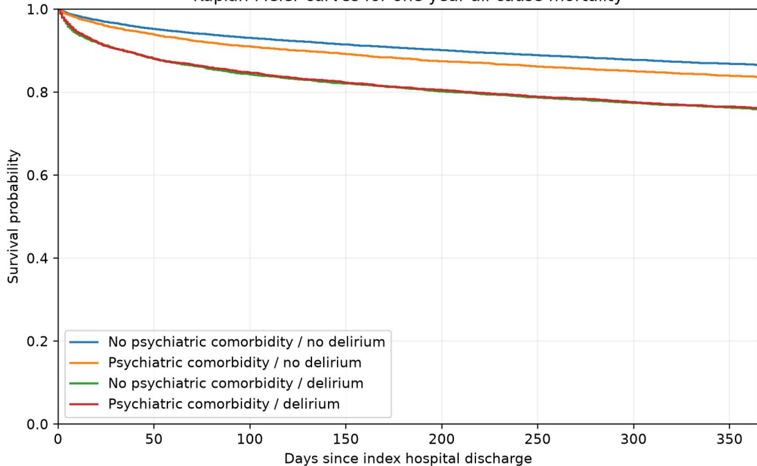
Kaplan-Meier curves for one-year all-cause mortality
