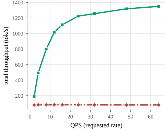
(c) Throughput vs QPS
