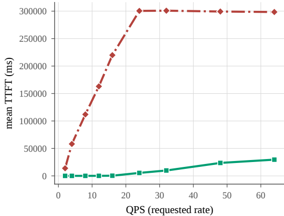
(a) TTFT vs QPS
