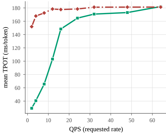
(b) TPOT vs QPS
