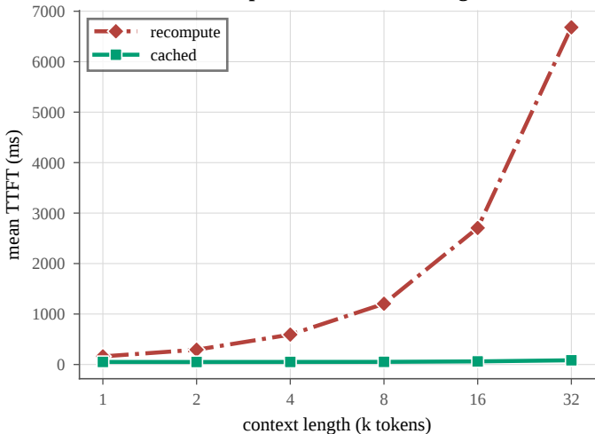
Recompute cost vs context length
