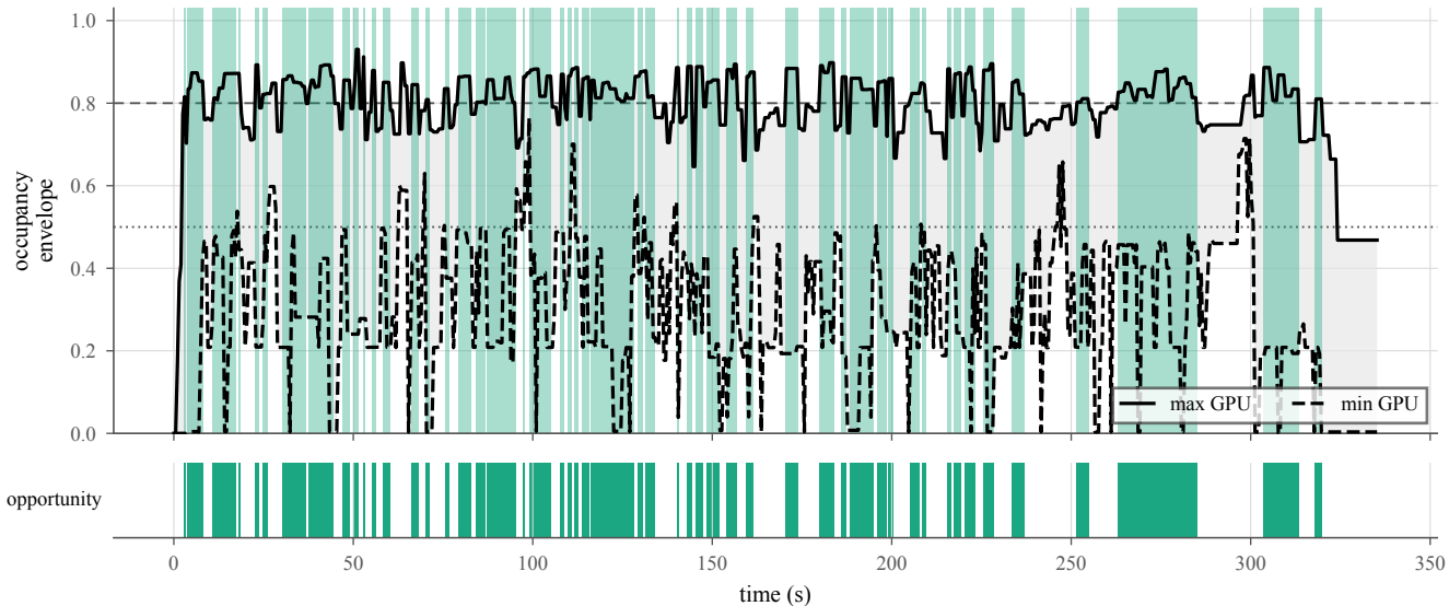
Opportunity: max GPU \geq 0.8 and min GPU \leq 0.5
