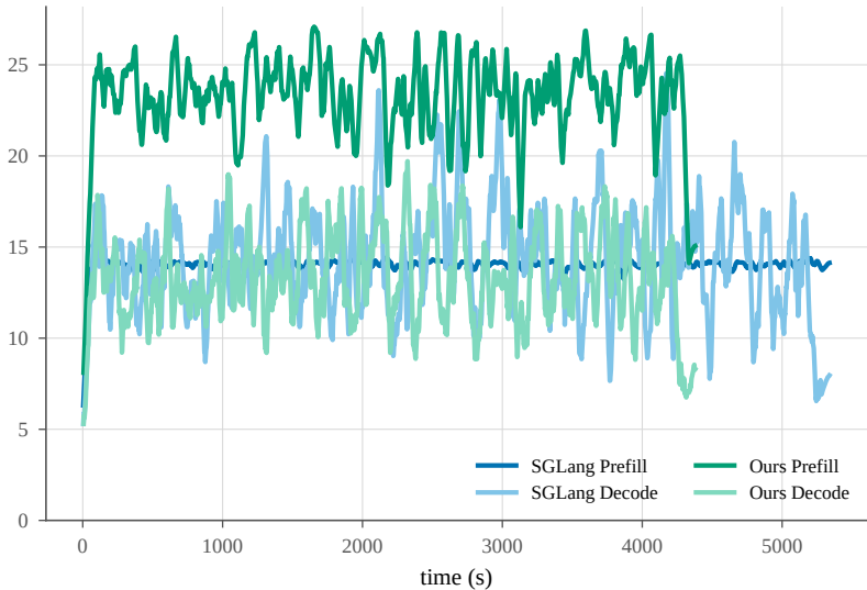
Resident KV (GB) (rolling mean, 15 samples)
