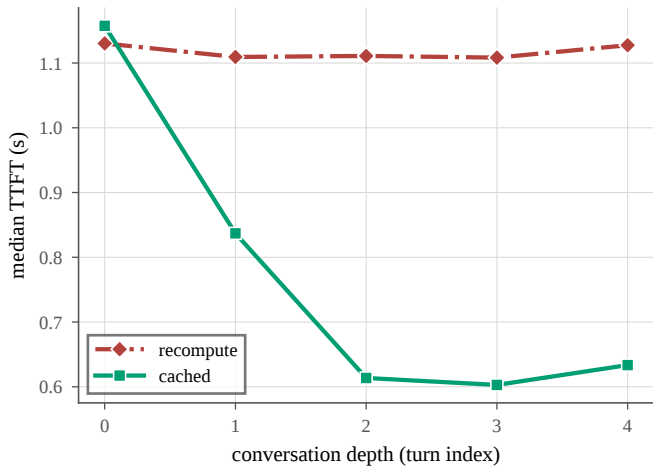
TTFT (lower is better)
