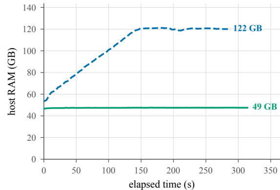
host RAM (lower better)
