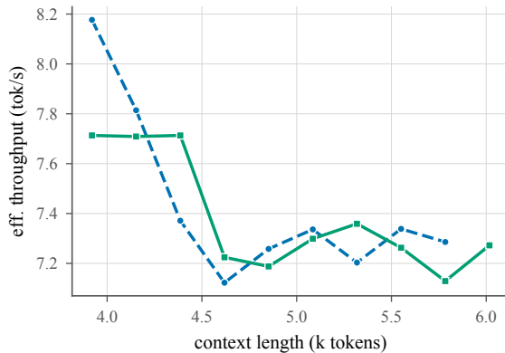
(a) BFCL v3
