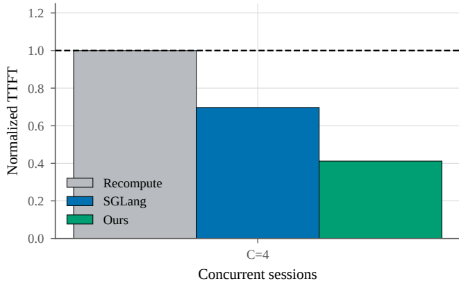
(a) Time to first token
