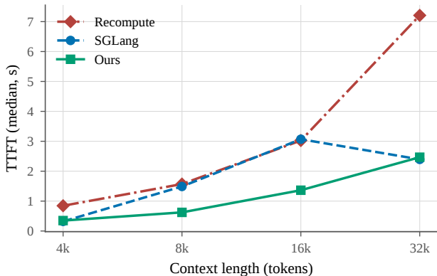
Time to first token vs context length
