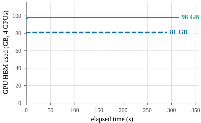
(a) GPU HBM footprint
