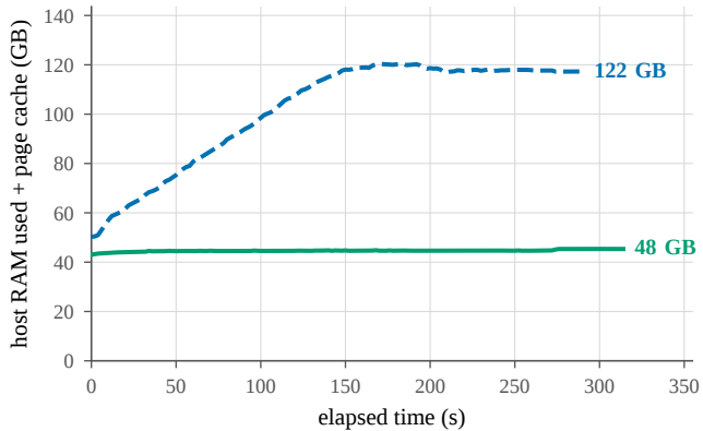
(b) host RAM footprint
