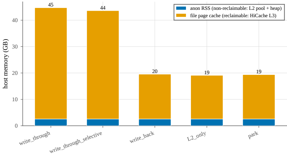
(a) Host RAM: real allocation vs reclaimable cache
