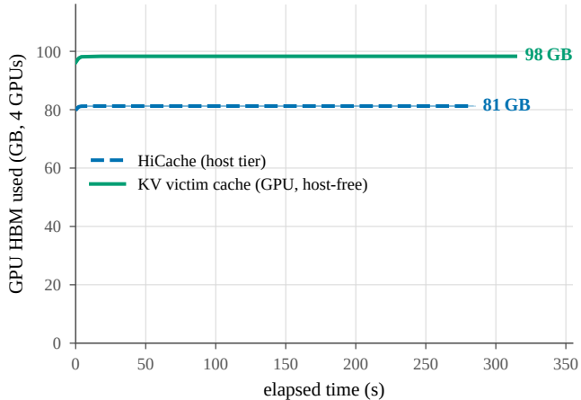
(a) GPU HBM footprint
