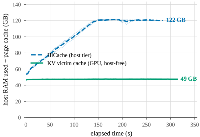
(b) host RAM footprint
