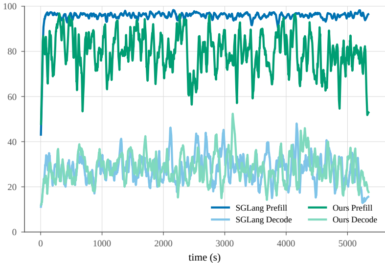
KV pool occupancy (%) (rolling mean, 15 samples)
