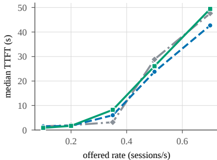
(b) Latency
