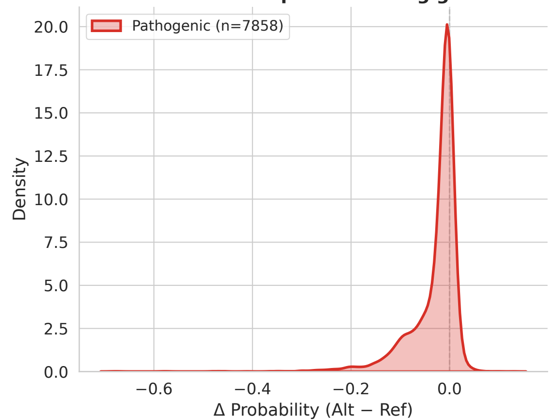
Frameshift — protein coding gene
