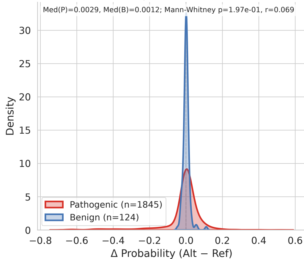
Splicing — exon
