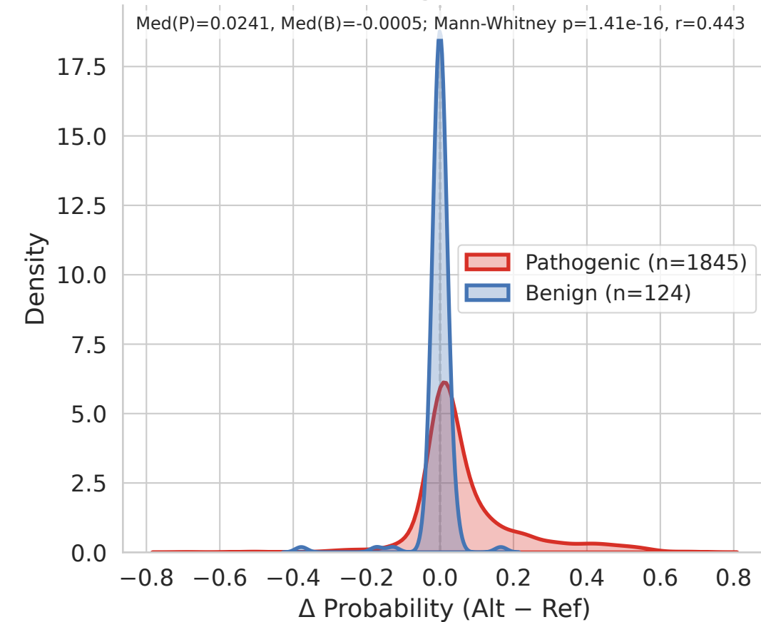
Splicing — intron
