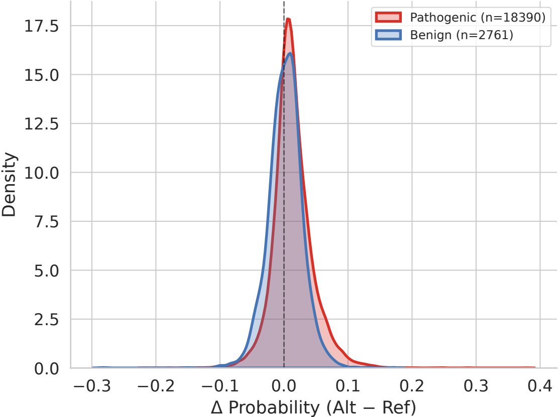
stop codon
