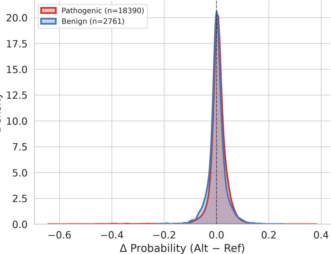
start codon
