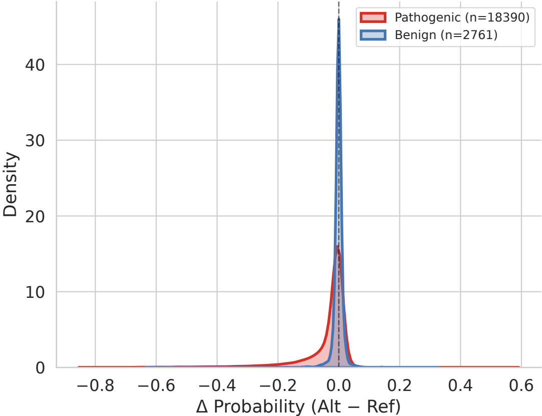
exon
