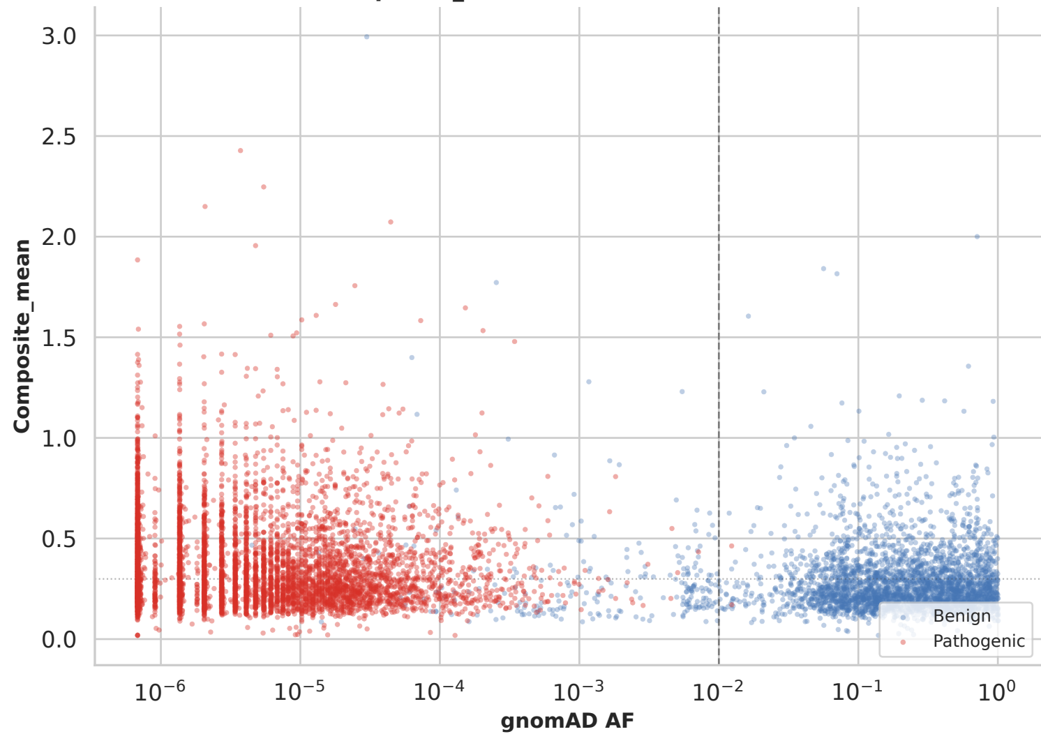
Composite_mean (AUC=0.687, d=0.54)
