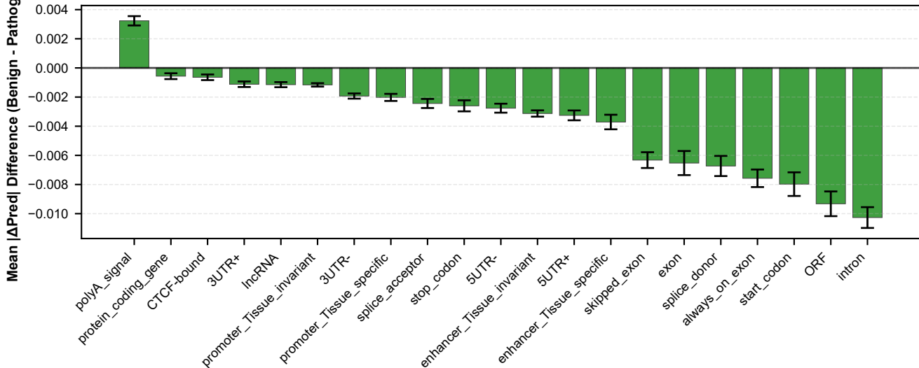
Per-Element Disruption: Benign vs Pathogenic (95% CI) Green = Significant (Bonferroni-corrected), n=21 elements
