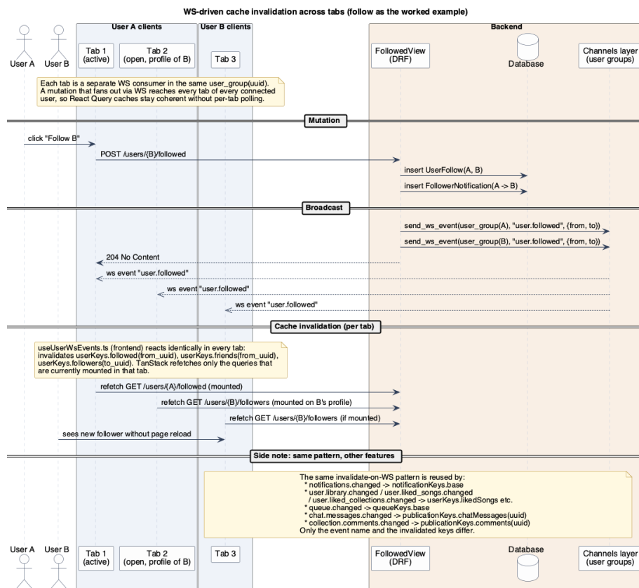
Figure C.27: WebSocket cache invalidation on follow mutation
