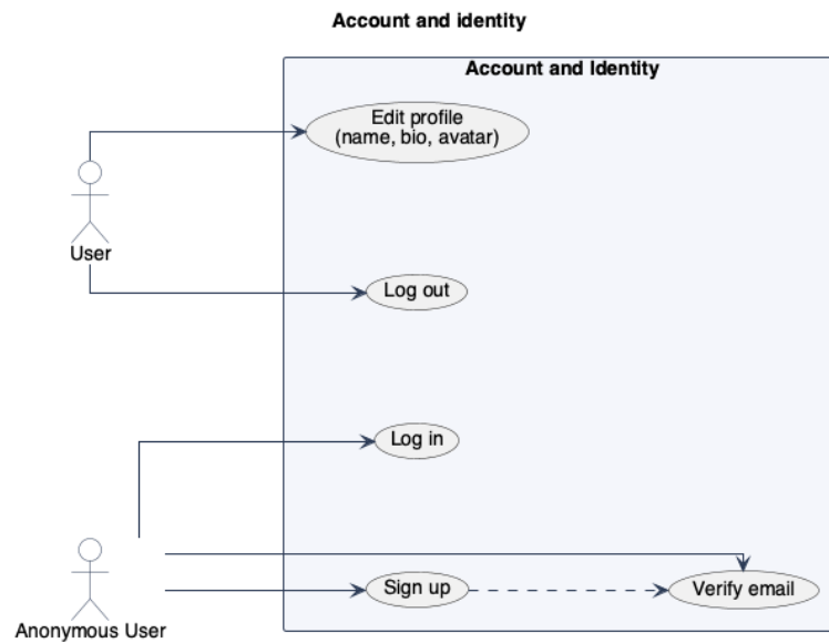
Figure C.4: Use cases: Account and Identity
