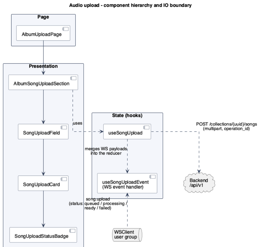
Figure C.21: Frontend component hierarchy: Audio Upload
