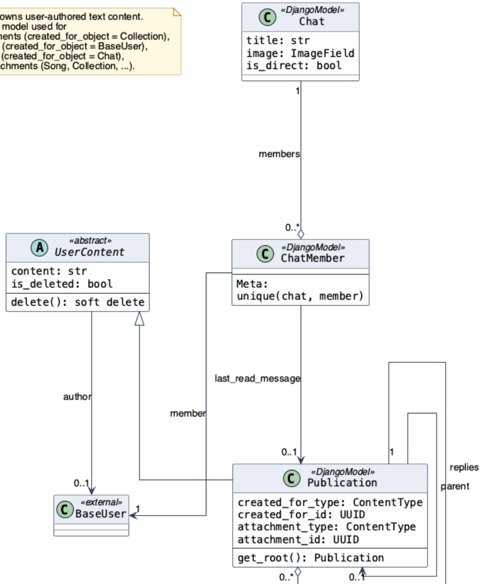
Figure C.16: Class diagram: Social (Publications, Comments, Chats)
