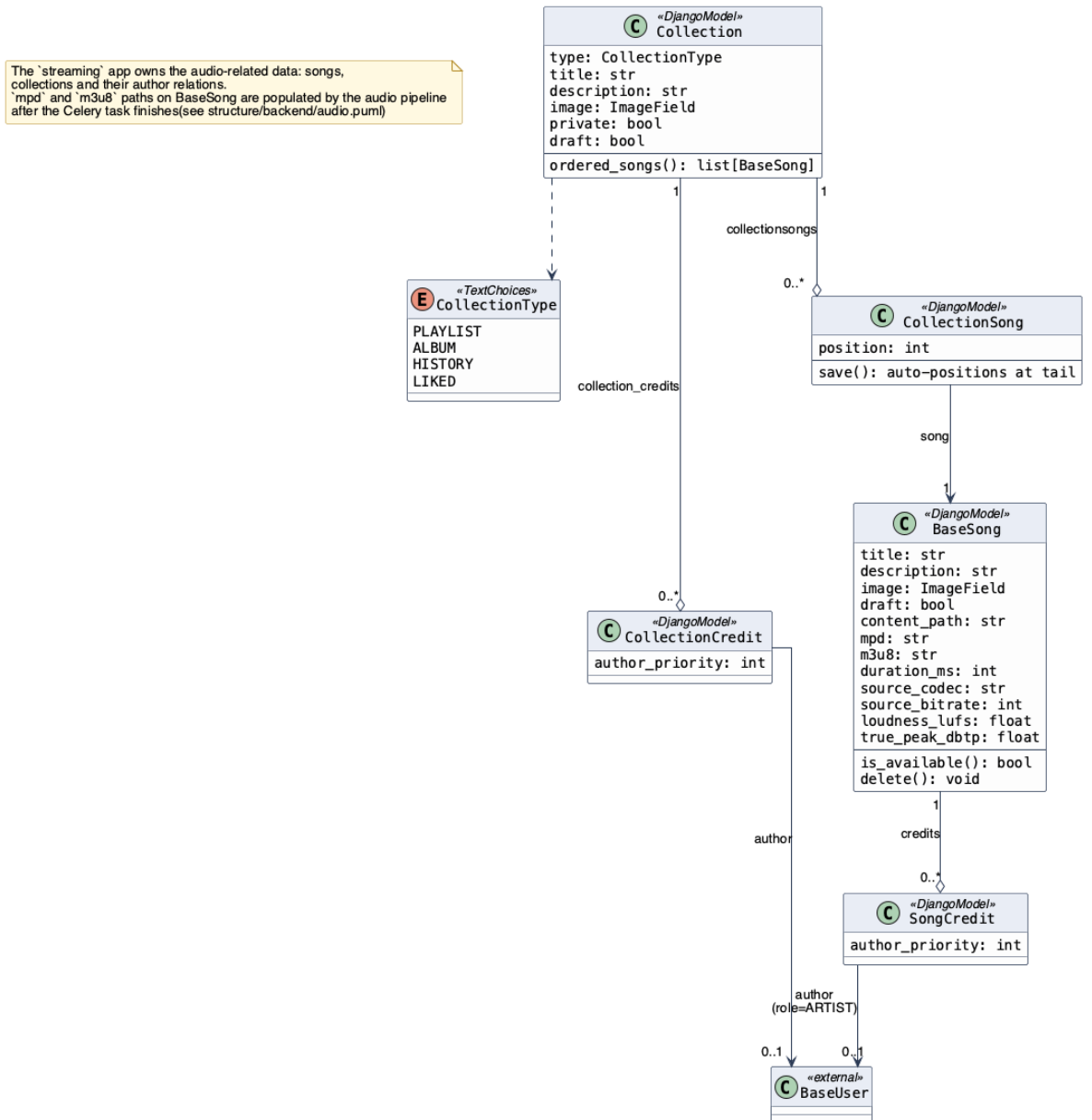
Figure C.11: Class diagram: Streaming (Songs, Collections, Credits)
