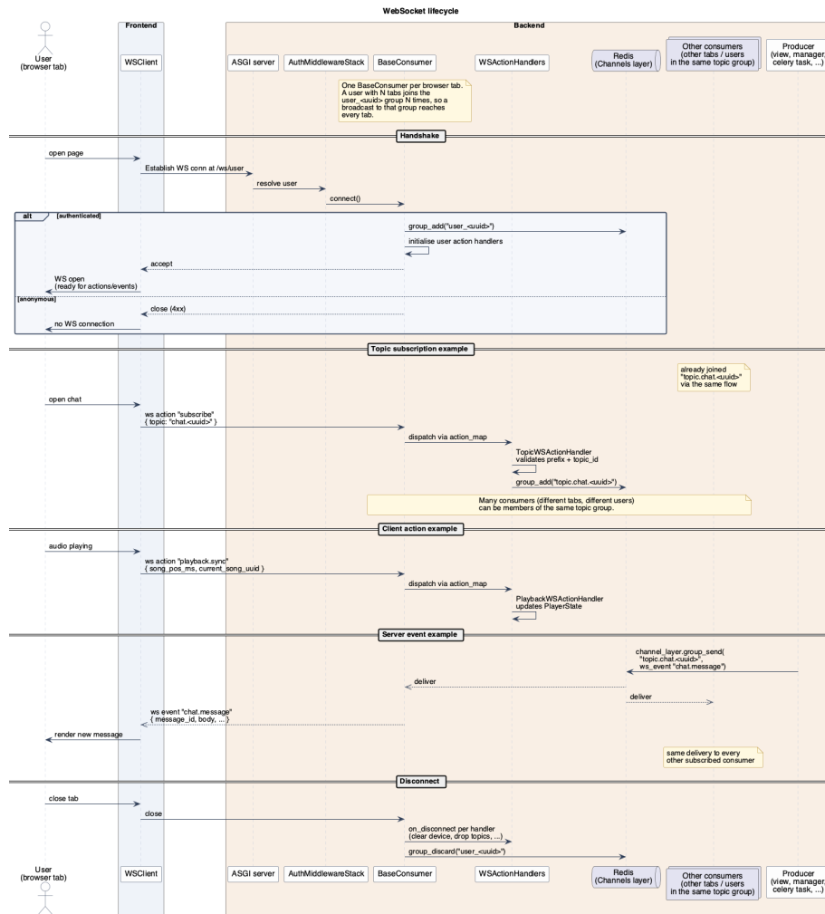
Figure C.26: WebSocket connection lifecycle
