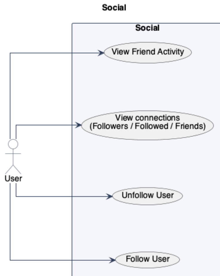
Figure C.5: Use cases: Social
