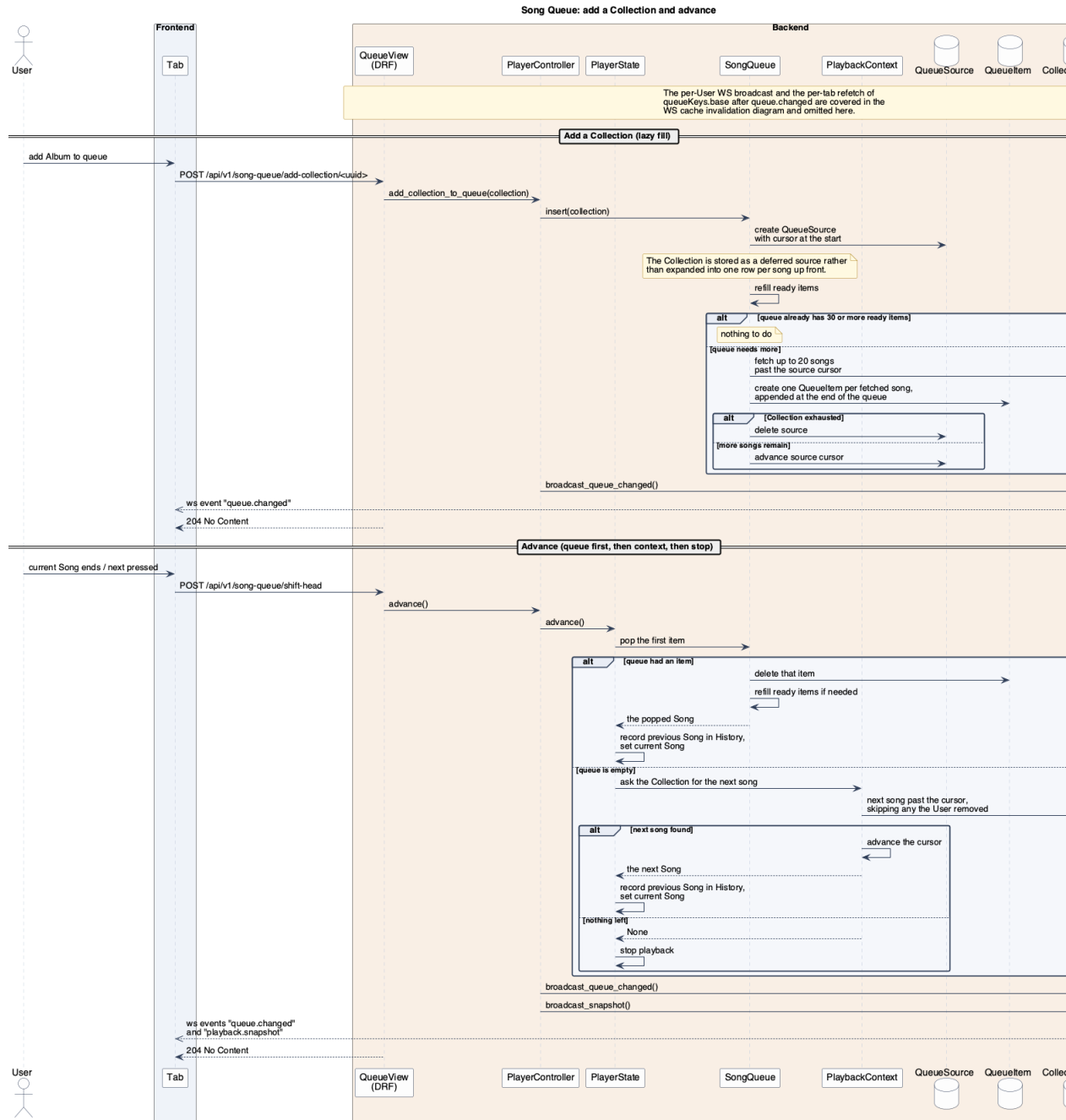
Figure C.31: Song Queue: add a Collection and advance
