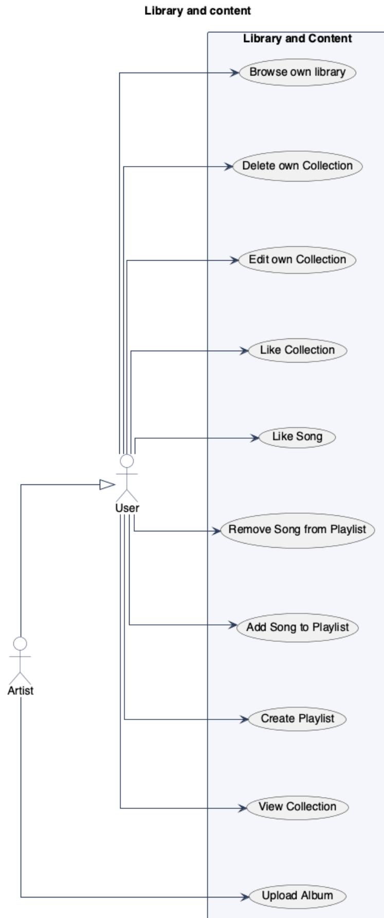
Figure C.6: Use cases: Library and Content
