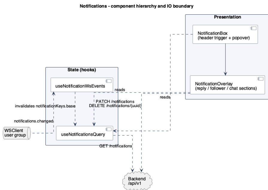
Figure C.25: Frontend component hierarchy: Notifications
