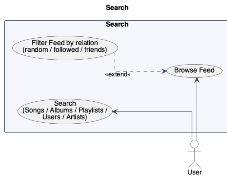
Figure C.8: Use cases: Search
