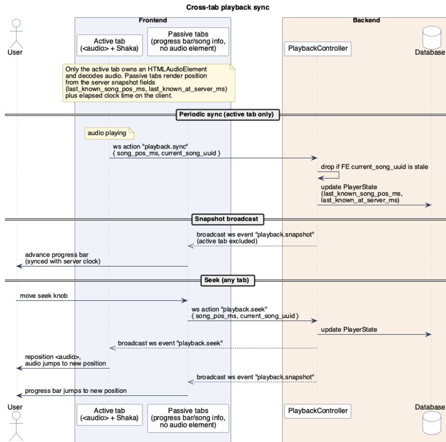
Figure C.30: Multi-tab playback synchronization
