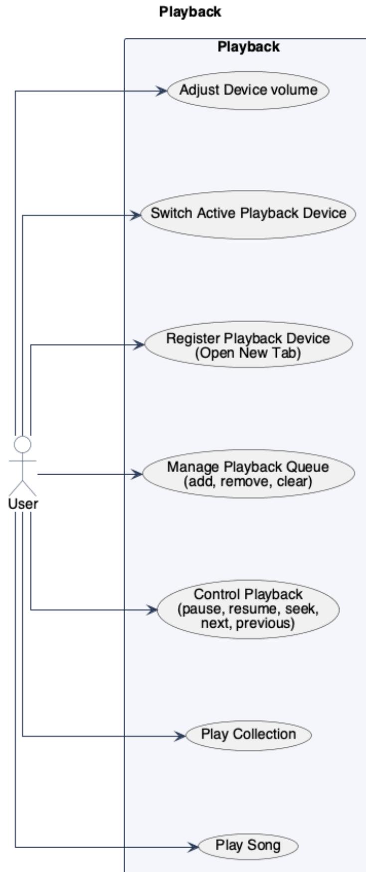
Figure C.7: Use cases: Playback
