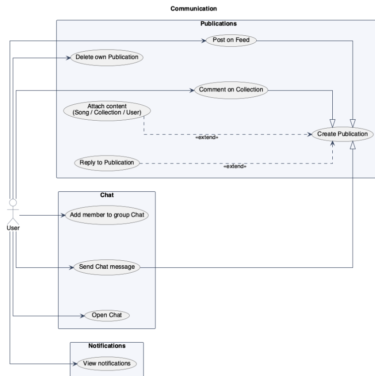
Figure C.9: Use cases: Communication
