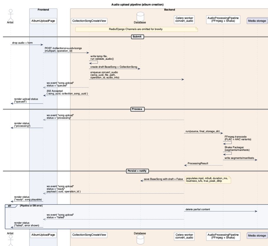
Figure C.29: Audio upload sequence
