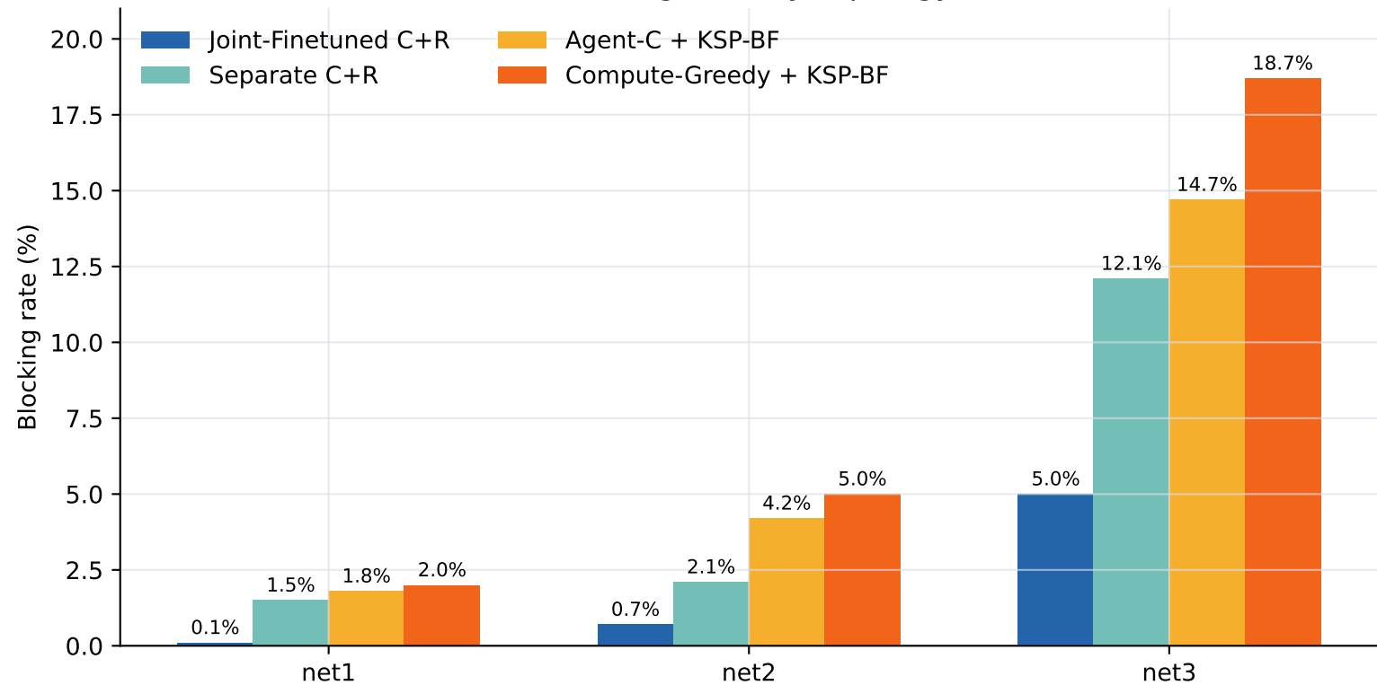
Blocking Rate by Topology
