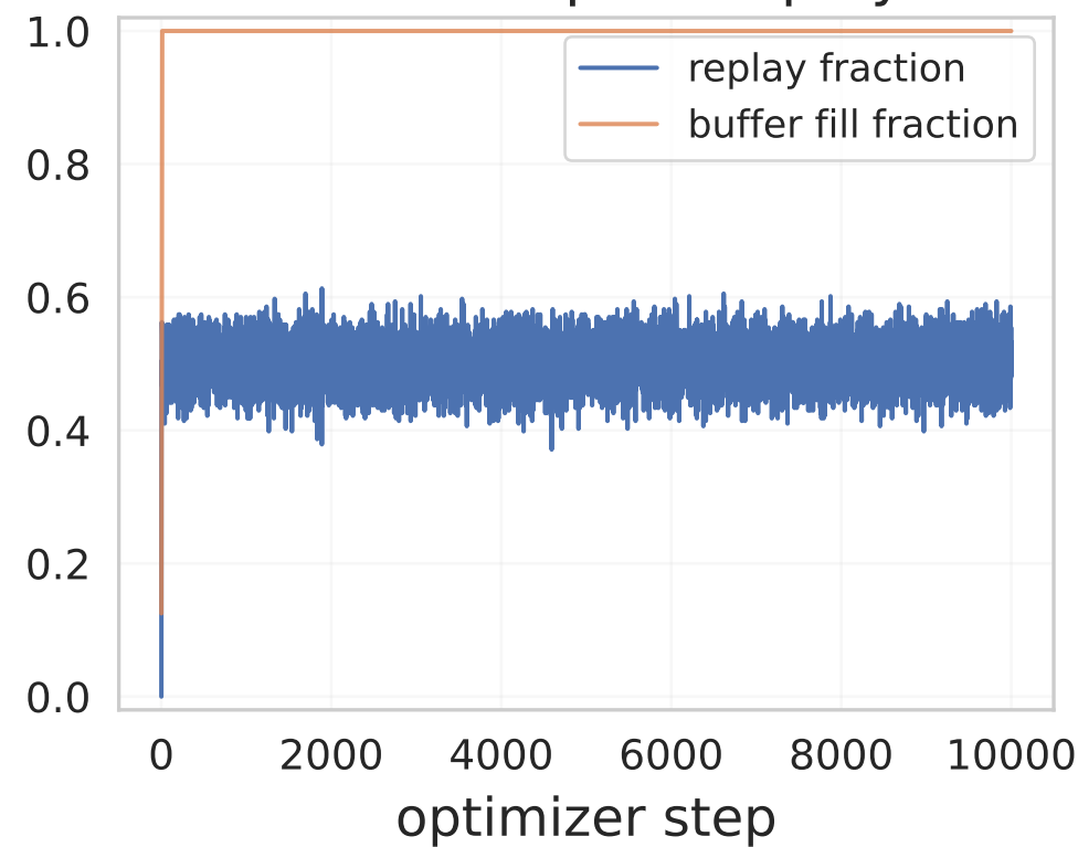
Historical-prior replay
