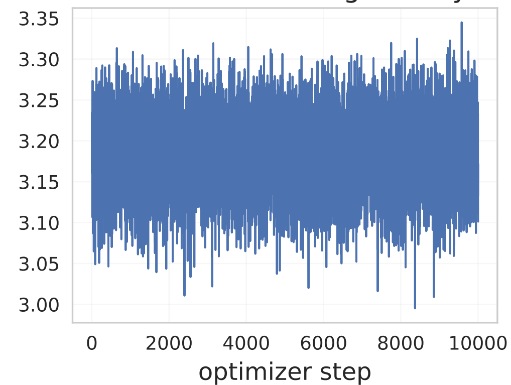
Mean likelihood log-density
