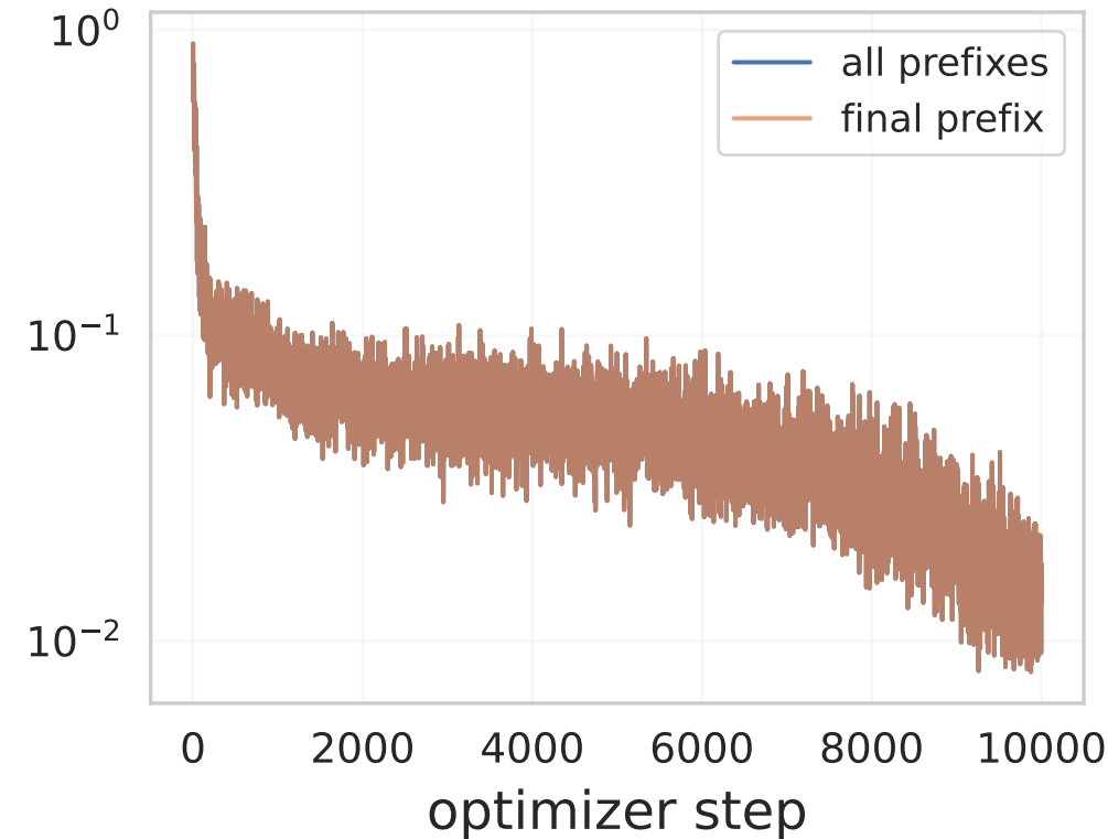
Historical-prior replay
