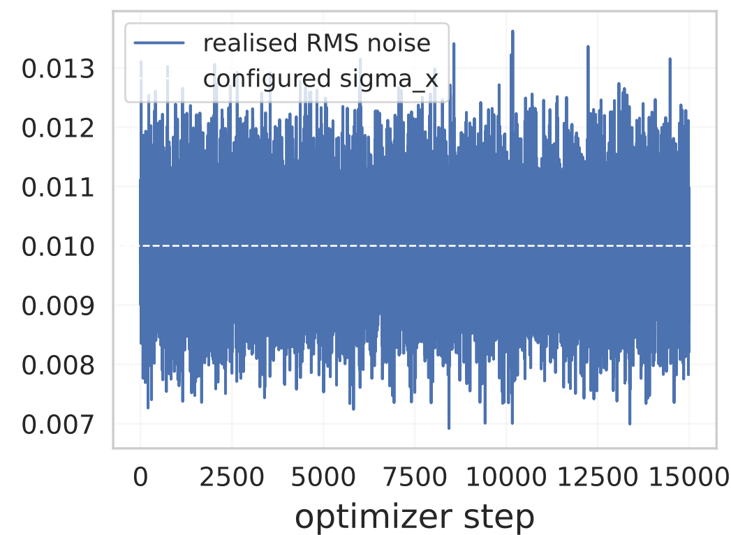
Gaussian x-likelihood noise
