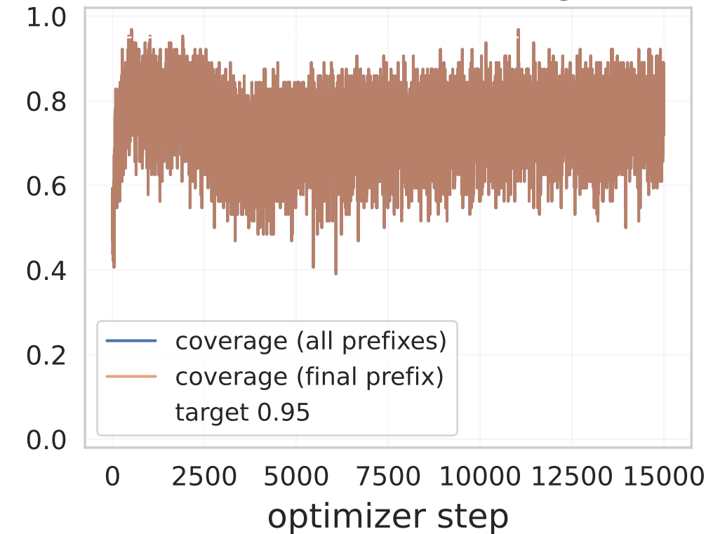
Gaussian x-likelihood noise
