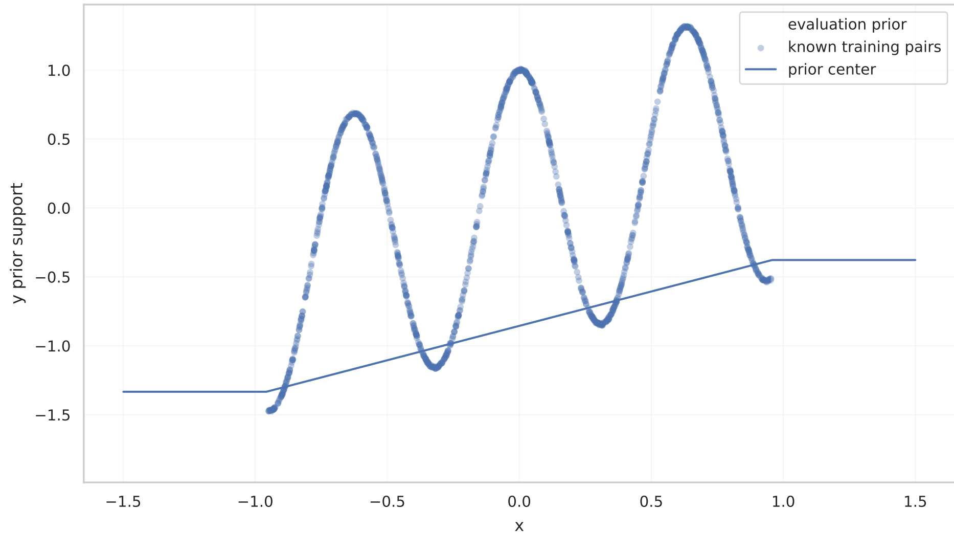
Evaluation prior support: nearest_training
