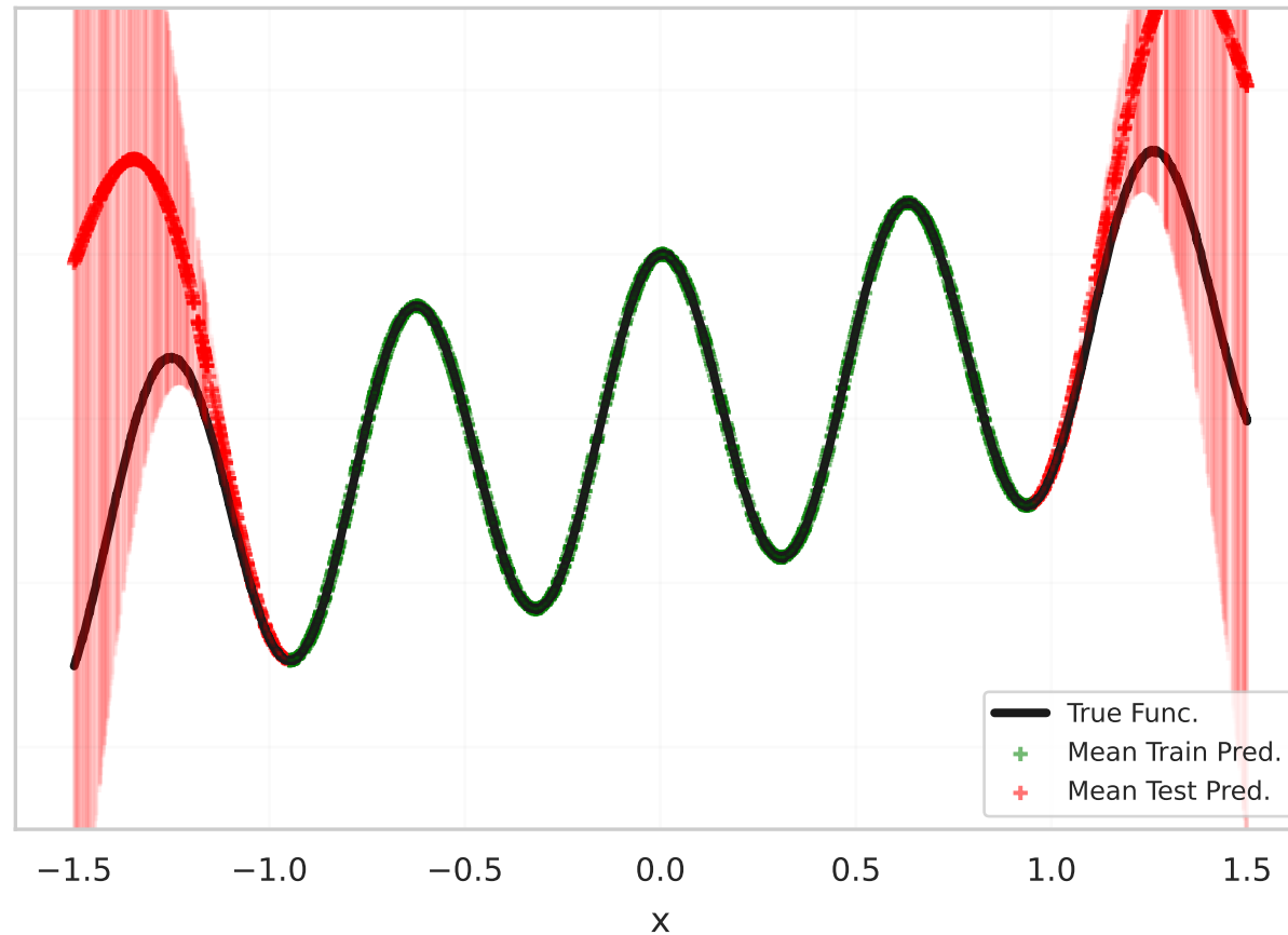
Gaussian Process
