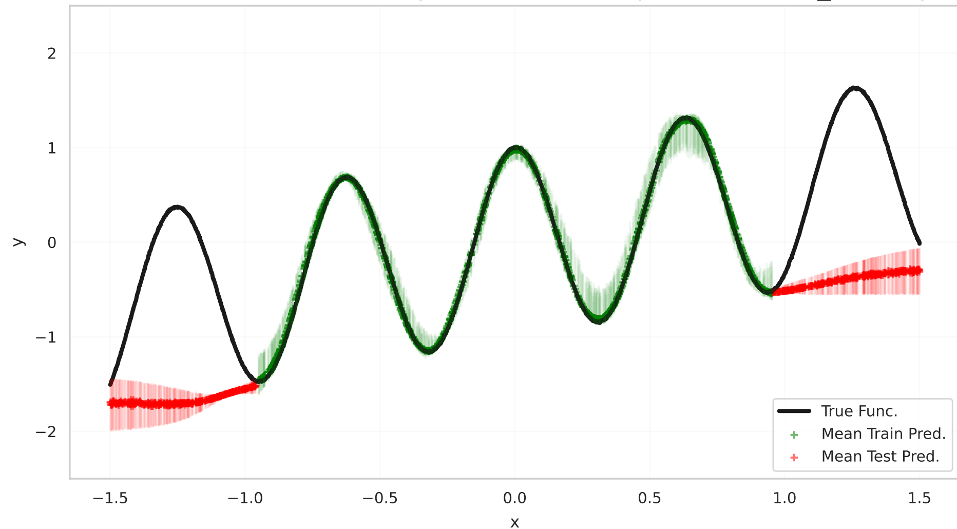
Conditional Particle Transport (adaln; test prior=nearest_training)
