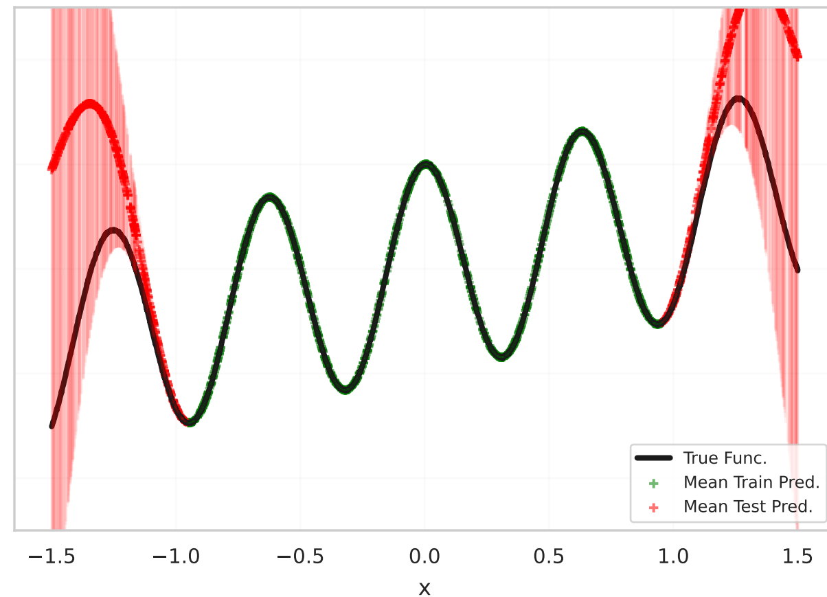
Gaussian Process
