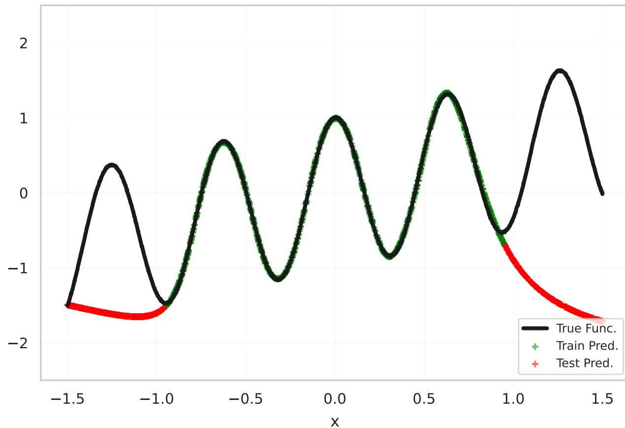
Standard MLP
