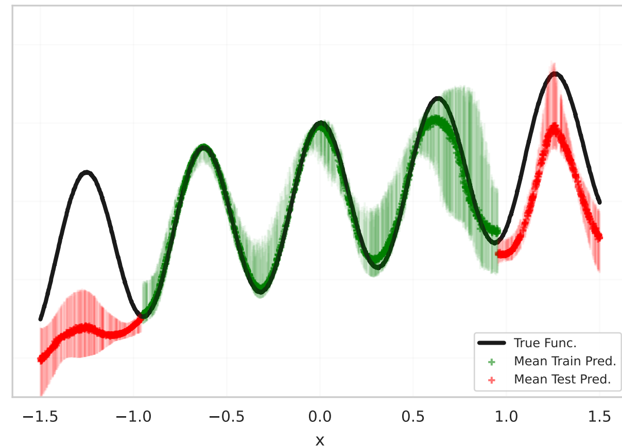
Particle Transport (adaln; test prior=cheating)
