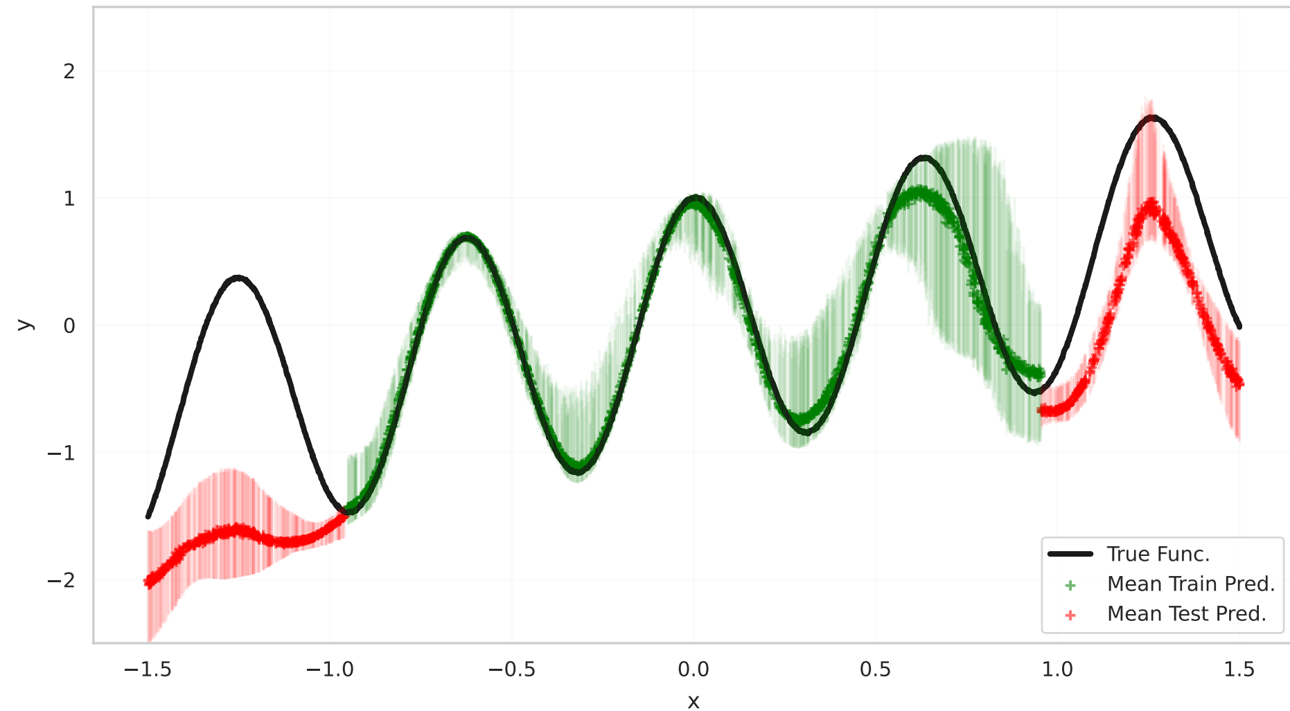
Conditional Particle Transport (adaln; test prior=cheating)
